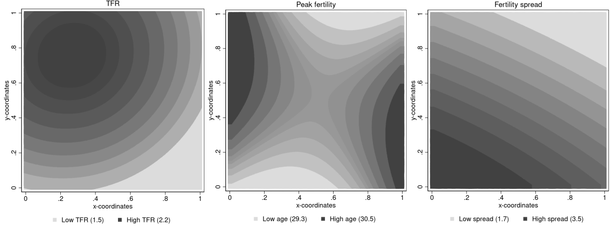
Figure 1: Simulated geographic distribution of fertility characteristics
