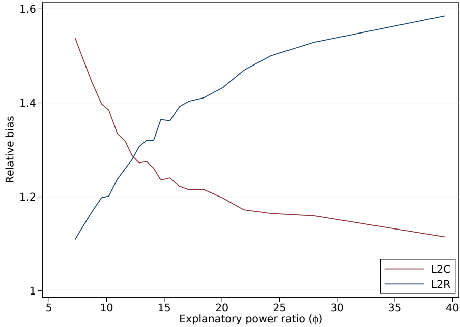
Figure 4: Relative bias and regional variation
