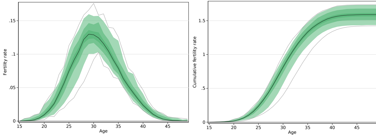
Figure 6: Distribution of empirical Bayes predictions of age-specific fertility rates across municipalities
