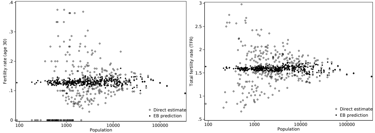
Figure 5: Fertility rates for municipalities of different sizes. Comparison of direct estimates and empirical Bayes predictions
