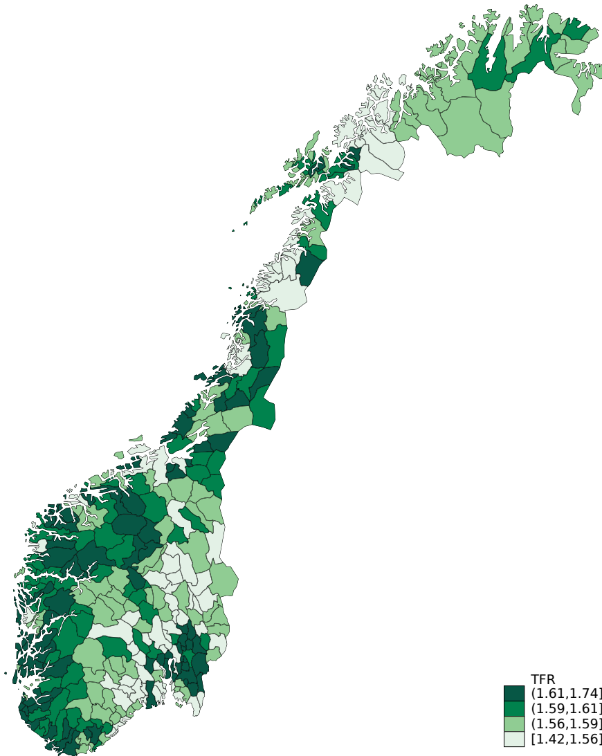
Figure 7: Geographic distribution of total fertility rates estimated by the empirical Bayes method
