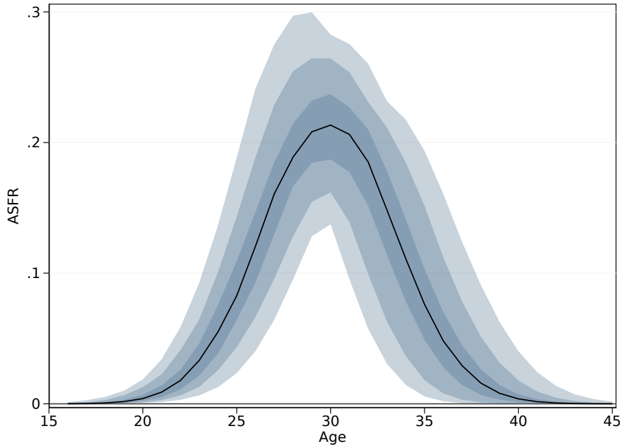
Figure 2: Simulated age-specific fertility rates
