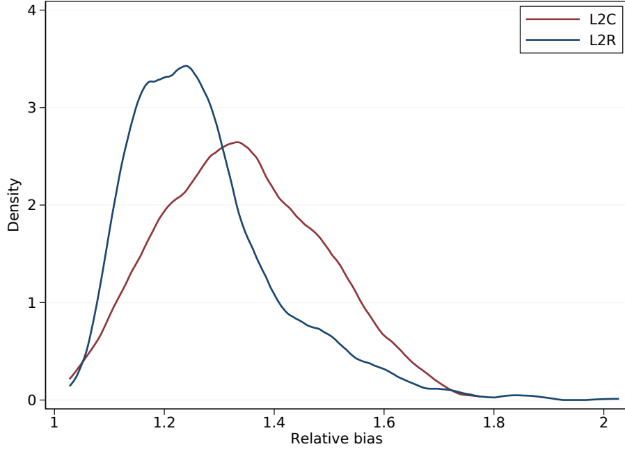
Figure 3: Distribution of relative bias
