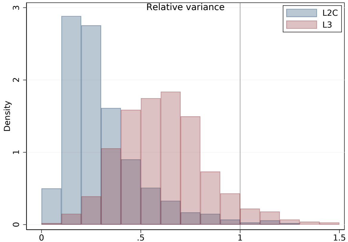
Figure B2: Overshrinkage of the empirical Bayes predictions
