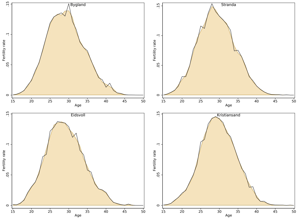
Figure C1: Comparison of smoothed and unsmoothed EB estimates of age-specific fertility rates in selected municipalities of different sizes
