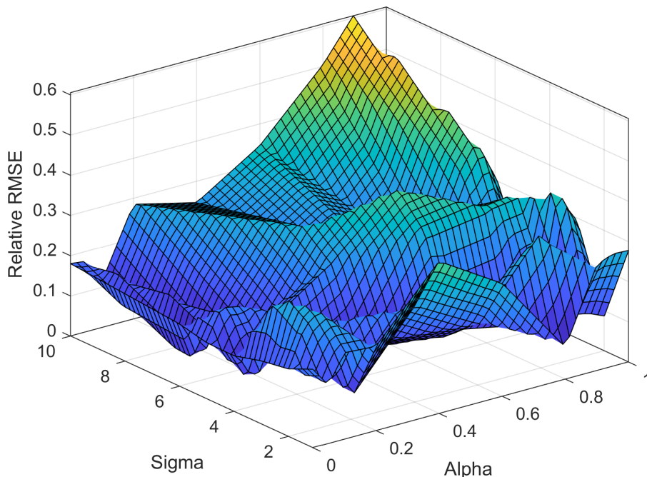
FIGURE 3: Relative RMSE. RMSE divided by the RMSE from the F/S estimator, see Soderbery (2015).
