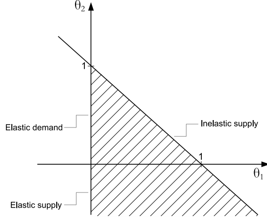
FIGURE 1: The admissible parameter space. The boundary \{\theta : \theta_1 > 0 \cap \theta_1 + \theta_2 = 1\} corresponds to inelastic supply ( \alpha = 1 ), \{\theta : \theta_1 = 0 \cap \theta_2 < 0\} to elastic supply ( \alpha = 0 ) and \{\theta : \theta_1 = 0 \cap 0 \leq \theta_2 \leq 1\} to elastic demand ( \sigma = \infty ).
