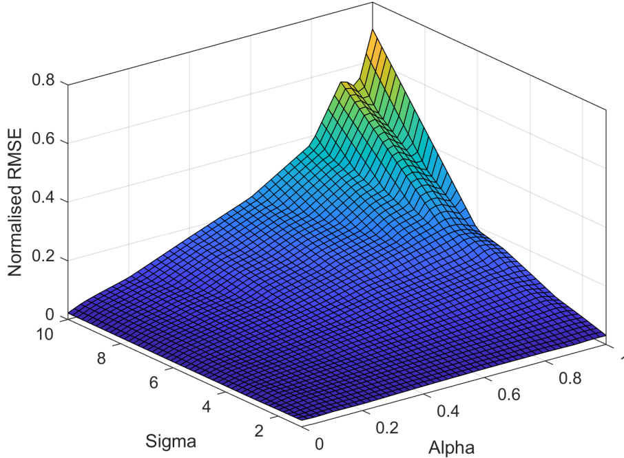
FIGURE 2: Normalised RMSE. RMSE divided by |\beta| = \sigma - 1
