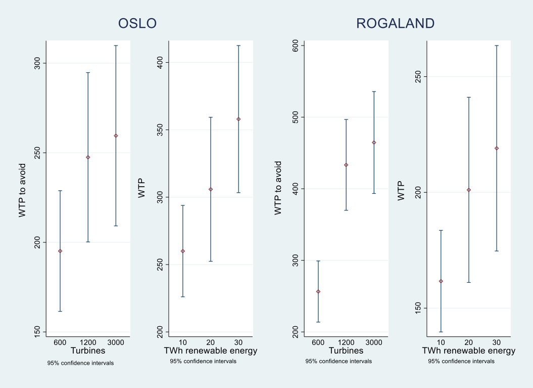
Figure 3: WTP per household per month (mean and 95% CI) by geographic subsample (Oslo and Rogaland counties) for the attributes TURB (number of turbines) and TWH (renewable electricity production in TWh) based on piecewise linear specification
