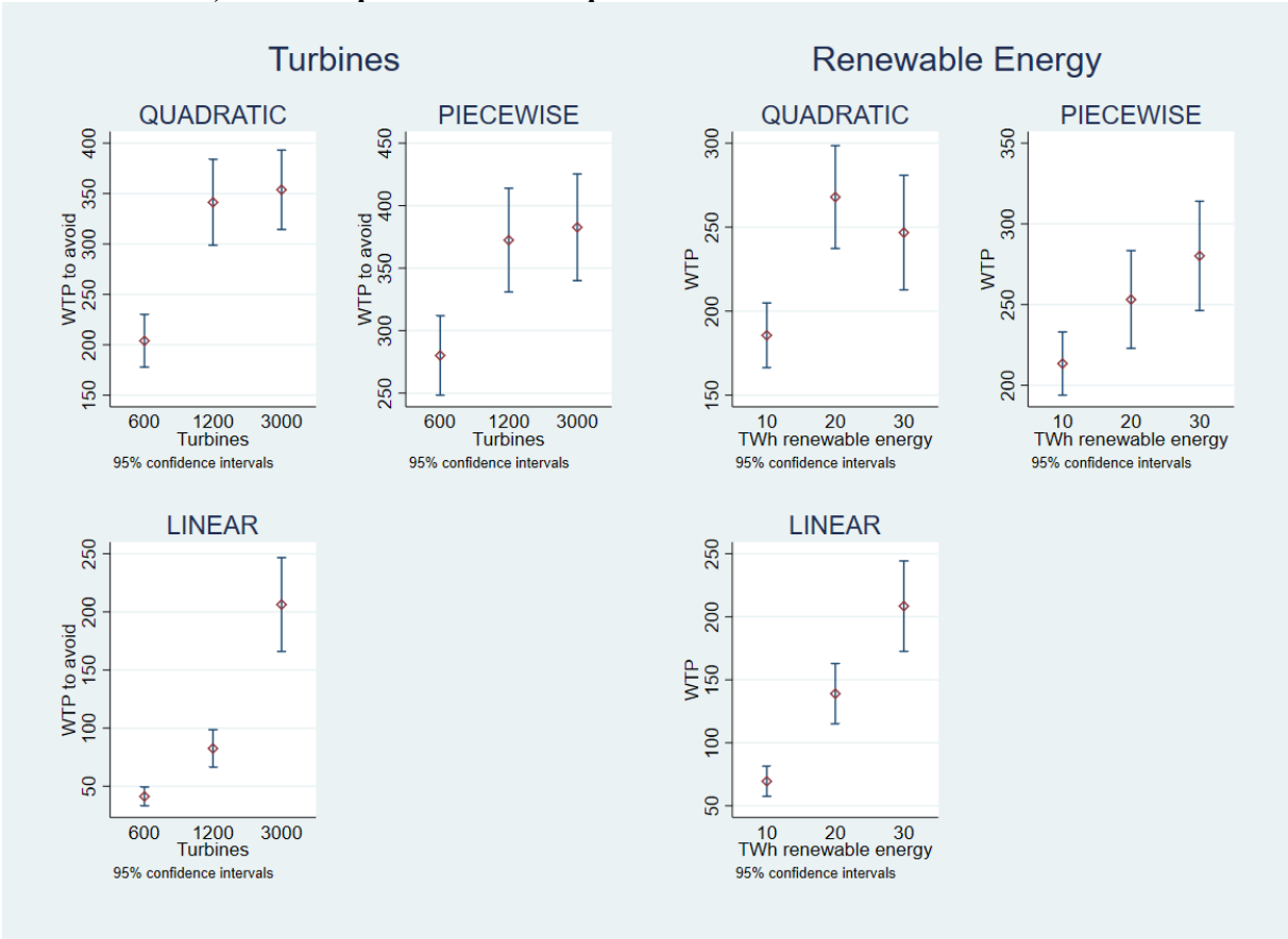
Figure 2: Full sample WTP per household per month (mean and 95% CI) for different functional forms for the attributes TURB (number of turbines) and TWH (renewable electricity production in TWh) based on piecewise linear specification
