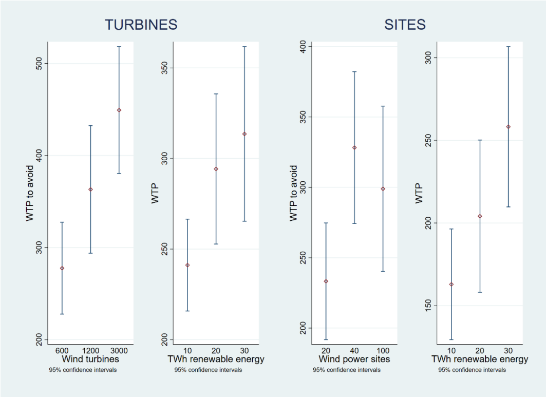
Figure 4: WTP per household per month (mean and 95% CI) by unit of measurement subsample (1 site = 30 turbines) for the attributes TURB (no. of turbines) and TWH (renewable electricity production in TWh) based on piecewise linear specification
