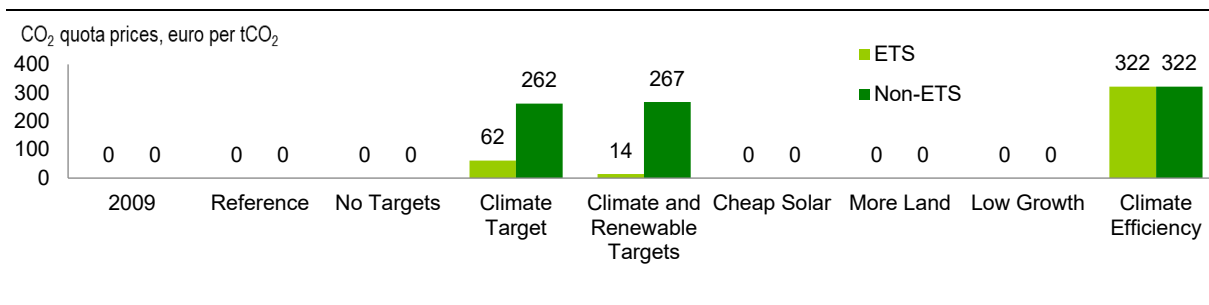
Figure 2 CO 2 prices in EU-30 in 2030 (€2009/tCO 2 )
