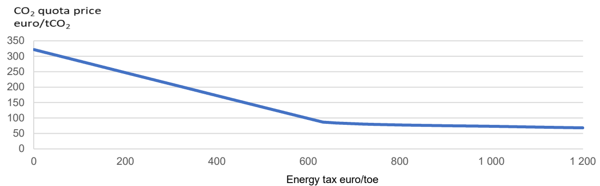
Figure 14 Equilibrium relationship between end-user tax on energy and CO 2 price when total emissions are fixed.
