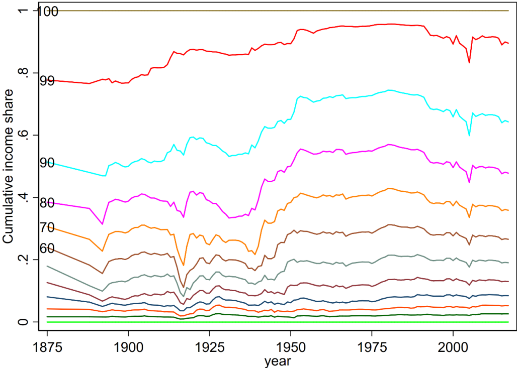
Figure A9. Top 1 and decile-specific shares of income in Norway, 1875-2017
