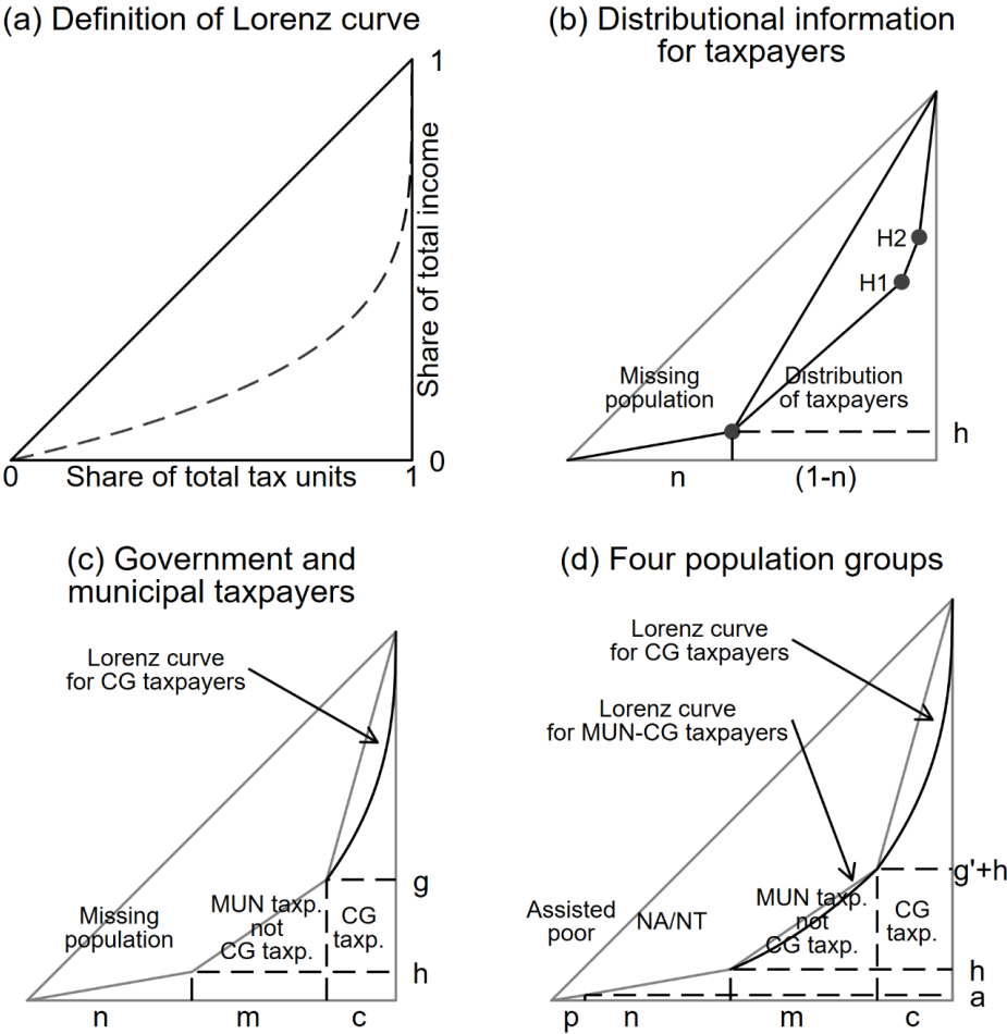
Figure 2. Estimation of Lorenz curves from tabular data
