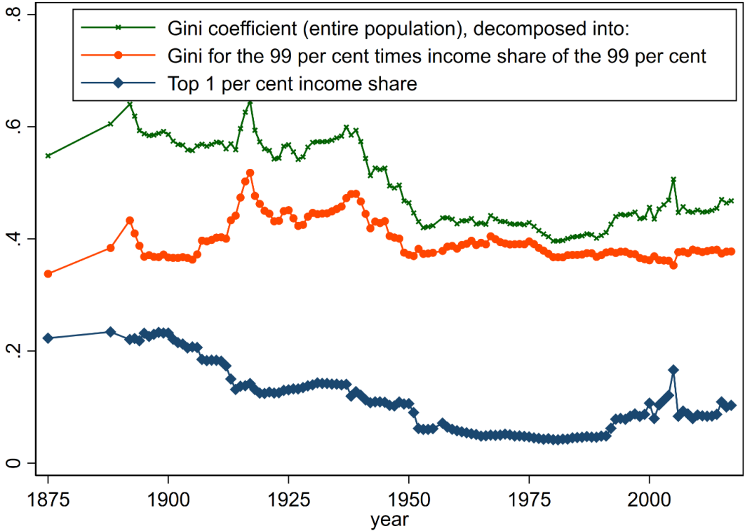
Figure 5. Decomposition of the Gini coefficient by the income share of the top 1 per cent and the Gini coefficient of the distribution of income among the bottom 99 per cent, Norway 1875 - 2017
