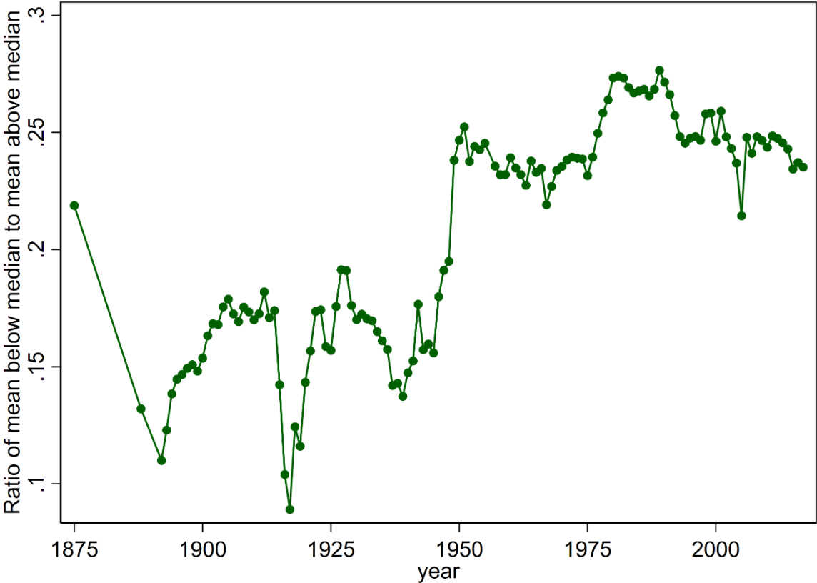
Figure A8. Mean income below the median relative to mean income above the median
