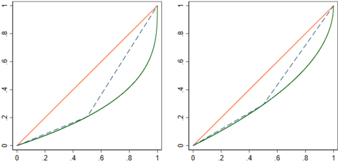
Figure A5. Illustration of Lorenz curves for Pareto distributions with shape parameter \alpha = 1.5 (left) and \alpha = 2 (right)
