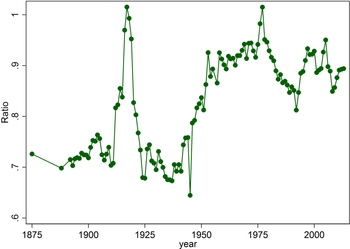
Figure A3. Internal total as a share of control total
