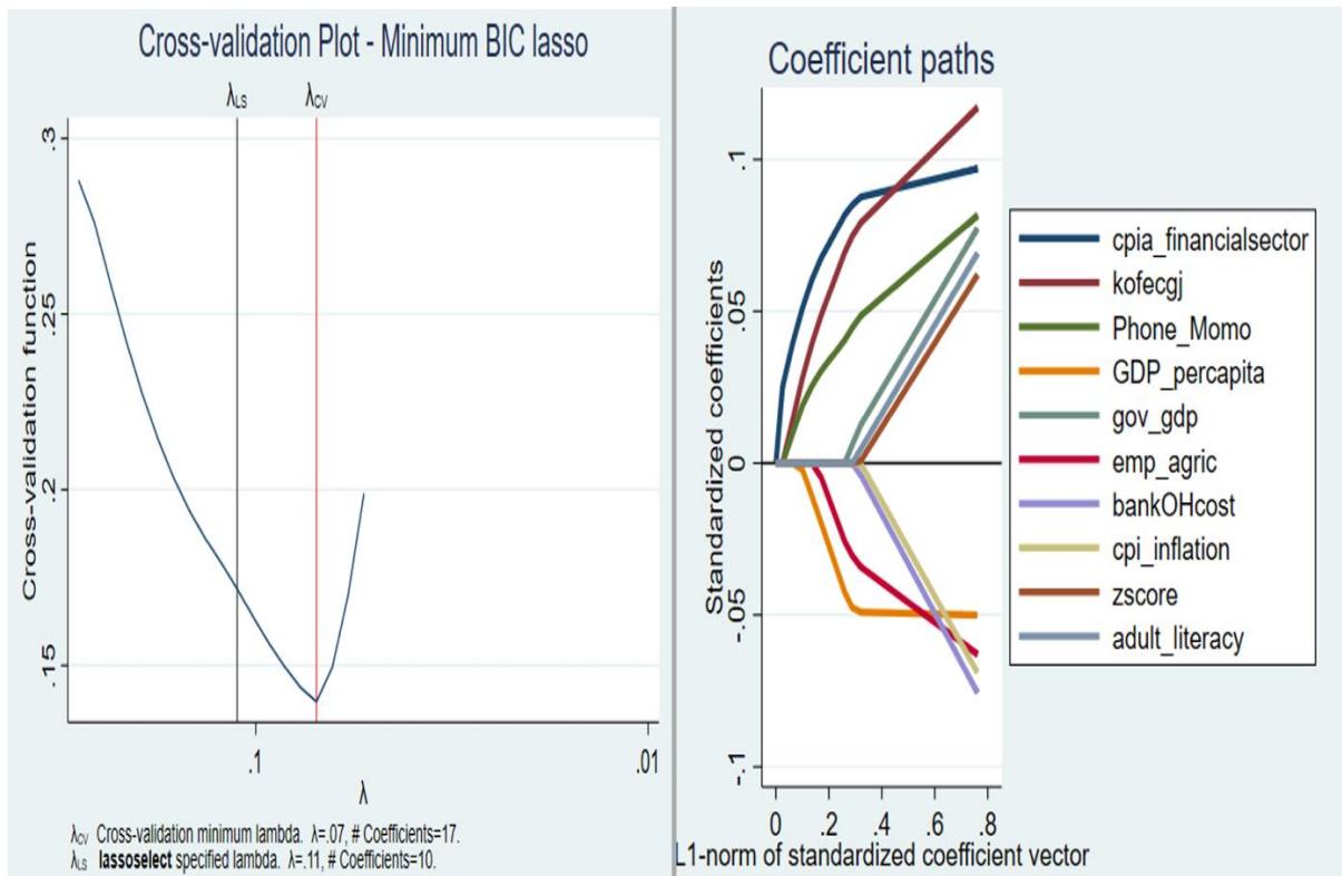
Figure 5: Cross-validation plot (left), and coefficient path plot (right) for Minimum BIC lasso
