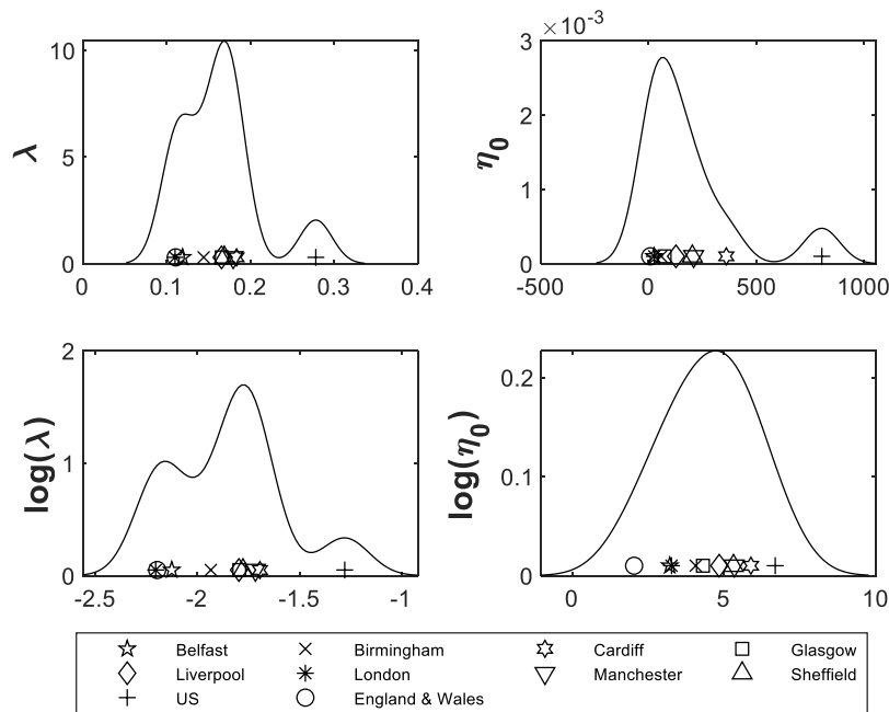
Figure B-7: Distribution of \eta_0 and \lambda implied by the models fitted to previous pandemics. Kernel density estimates.
