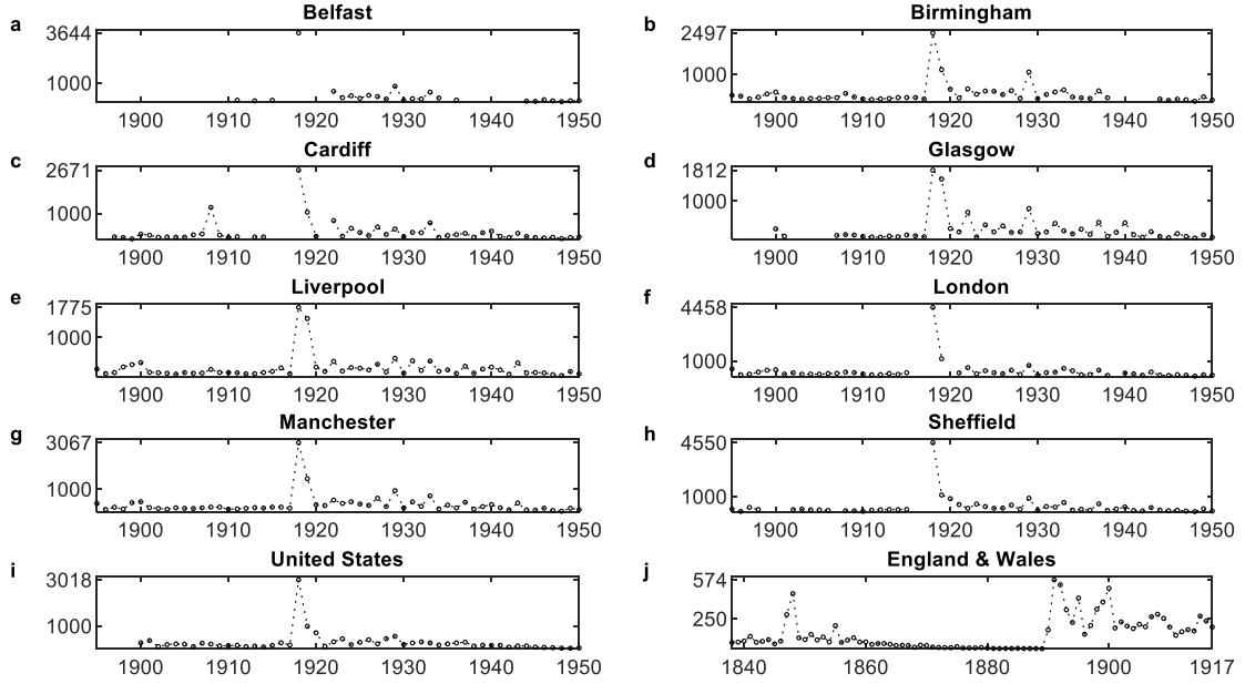
Figure 1. Annual mortality rate from influenza. Mortality rate in deaths per million population. The upper y-axis tick indicates the maximum mortality rate for each data series. Data for UK cities are taken from Medical Officer for Health reports. Data for the US are taken from Lindner and Grove (1943) and Grove and Hetzel (1968). Data for England & Wales are taken from Langford (2002), Table 5.
