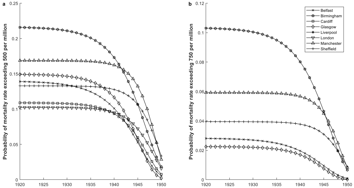
Figure B-4: Outbreak risk following the 1918-19 pandemic (model with estimated bounds). Outbreak probabilities computed from models fitted to each city. Upper and lower bounds are fitted to the data (1920-1950) for each city.
