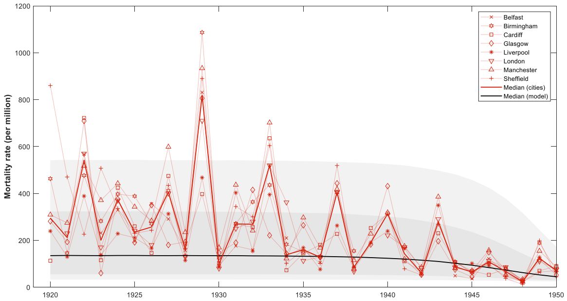
Figure B-3: Model predicted influenza mortality rates following the 1918-19 pandemic (model with estimated bounds). Simulated median (solid black line), interquartile range (dark shading) and 80% prediction interval (light shading) are based on 1m random draws. Simulated outcomes are based on the model fitted using the average across cities. Upper and lower bounds are fitted to the data. Data are overlotted in red. Data for UK cities are taken from Medical Officer for Health reports.
