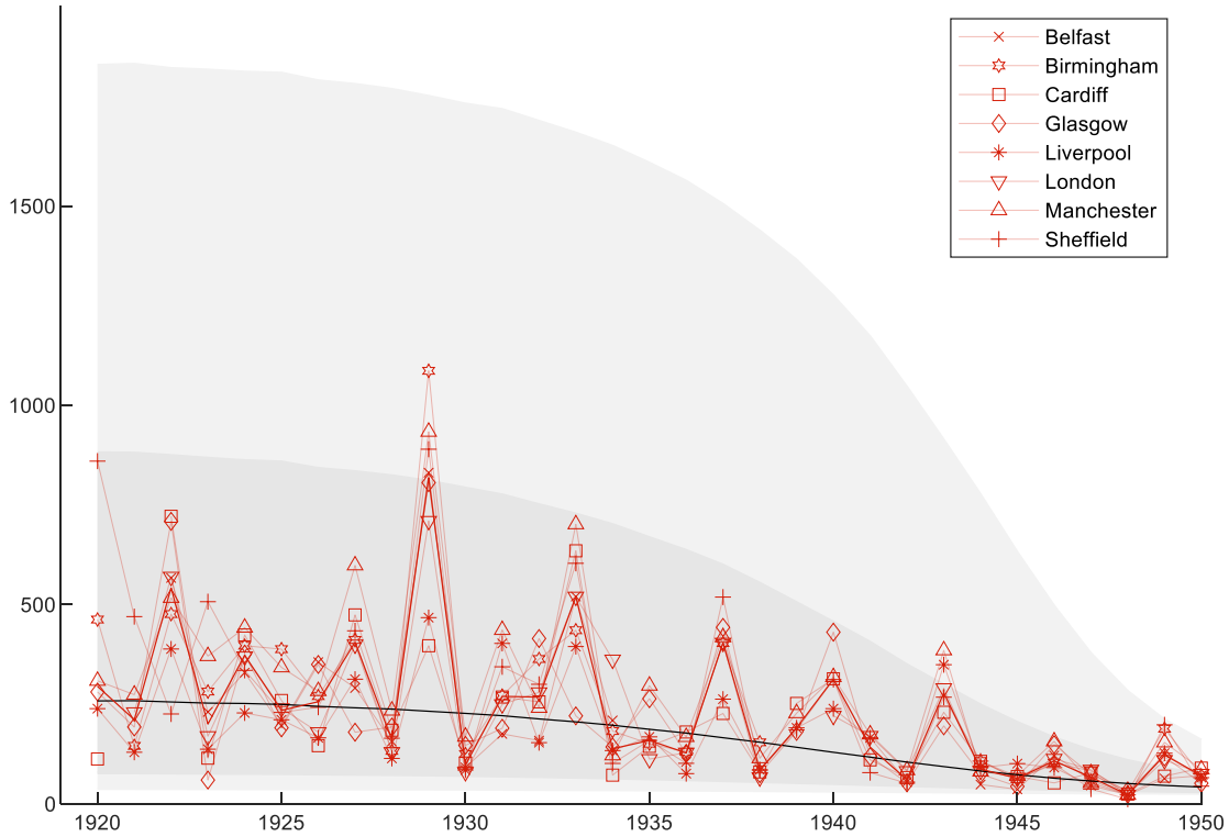
Figure 2: Simulated median (solid black line), interquartile range (dark shading) and 80% prediction interval (light shading), based on 1m random draws of the model fitted using the average mortality rates across cities, with data overplotted in red.
