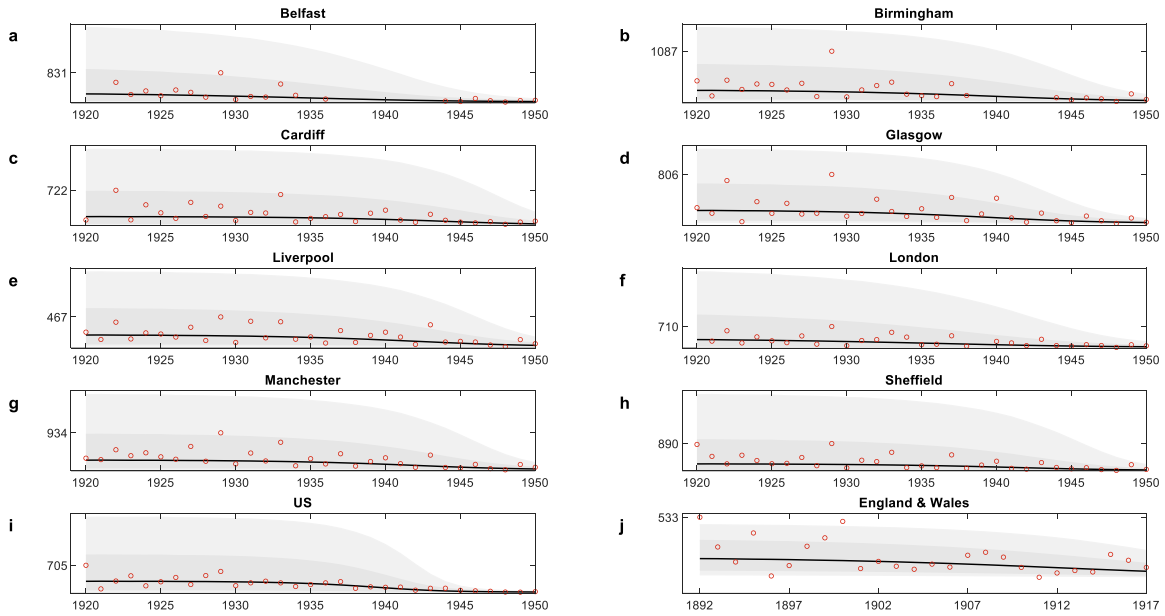
Figure C-1: Model predicted influenza mortality rates following the 1918-19 and 1890-91 pandemics (deaths per million). Simulated median (solid black line), interquartile range (dark shading) and 80% prediction interval (light shading) are based on 1m random draws. Simulated outcomes are based on the model fitted to each city, the US and England & Wales. Data for UK cities are taken from Medical Officer for Health reports. Data for the US is taken from Lindner and Grove (1943) and Grove and Hetzel (1968). Data for England & Wales are taken from Langford (2002), Table 5.
