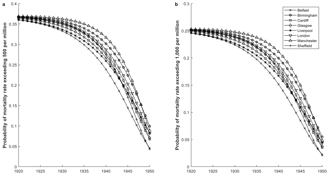
Figure B-1: Outbreak risk following the 1918-19 pandemic (model with common bounds). Outbreak probabilities computed from models fitted to each city. Upper and lower bounds are common and set to be the highest and lowest mortality rates within the sample of cities respectively.
