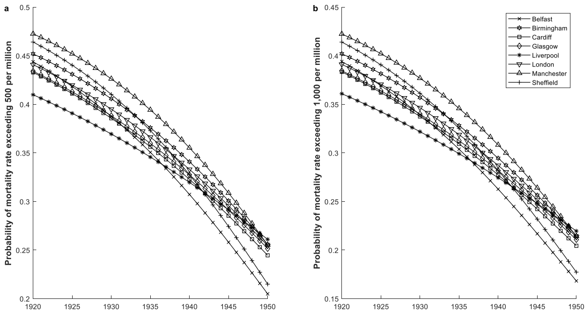
Figure B-2: Outbreak risk following the 1918-19 pandemic (model with theoretical bounds). Outbreak probabilities computed from models fitted to each city. Upper and lower bounds are set to 1,000,000 and 1 respectively.
