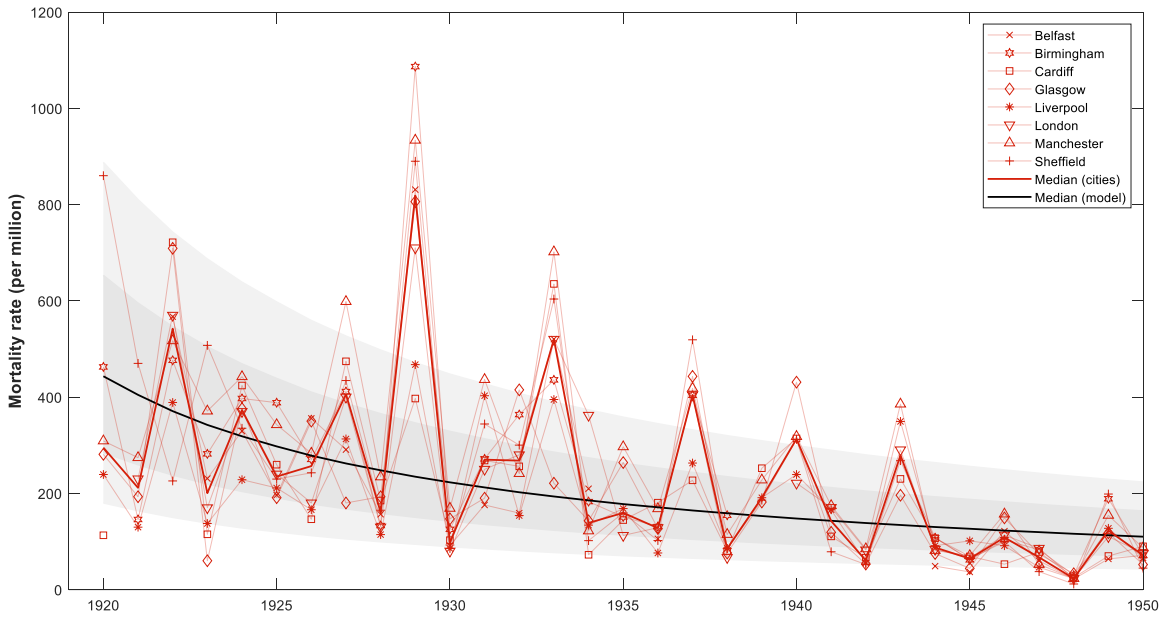
Figure B-5: Model predicted influenza mortality rates following the 1918-19 pandemic (One-parameter Weibull model). Simulated median (solid black line), interquartile range (dark shading) and 80% prediction interval (light shading) are based on 1m random draws. Simulated outcomes are based on the model assuming a sequence of one-parameter Weibull distributions fitted using the average across cities (1920-1950). Data are overplotted in red. Data for UK cities are taken from Medical Officer for Health reports.
