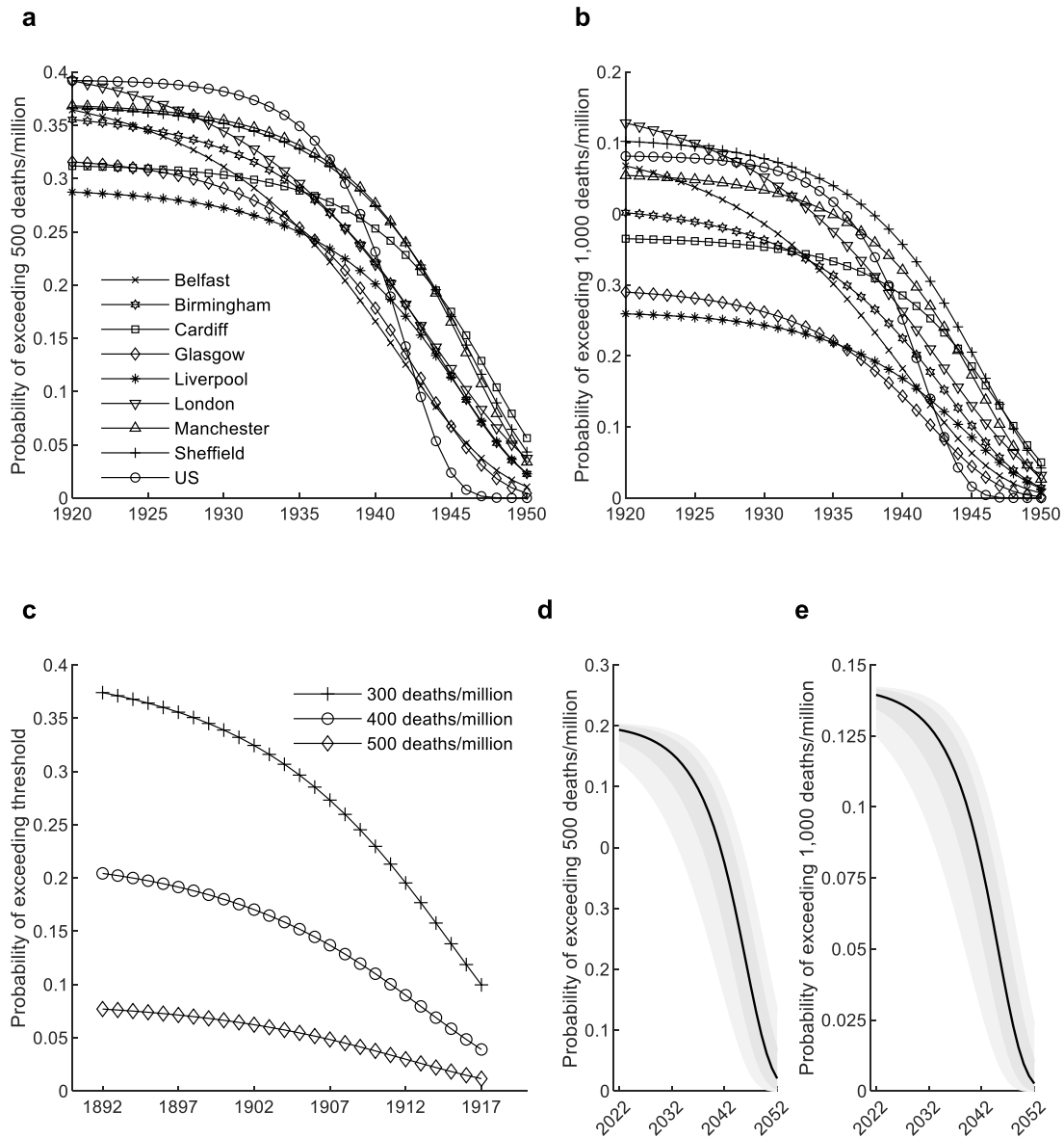
Figure 3. Outbreak risk following the historical 1918-19 and 1890-91 pandemics and COVID-19. (a)-(b) Outbreak probabilities computed from models fitted to each city and the US, for thresholds of (a) 500 deaths per million and (b) 1000 per million. (c) Outbreak probabilities computed from the model fitted to data for England and Wales following the 1890-91 pandemic, for different thresholds. (d)-(e) Simulated outbreak probabilities for COVID-19, showing median (solid black line), interquartile range (dark shading) and 80% prediction interval (light shading), based on 1m random draws. Outbreak probabilities are computed from model parameterisations that are drawn from a distribution of \eta_0 and \lambda implied by the models fitted to historical data. The upper bound on future mortality ( d_u = 1858 ) is set equal to COVID-19 mortality in the UK in 2020 and the lower bound ( d_l = 24 ) to reflect mortality in the non-pandemic state, approximated by background influenza mortality pre-2020 (data sources in SI).
