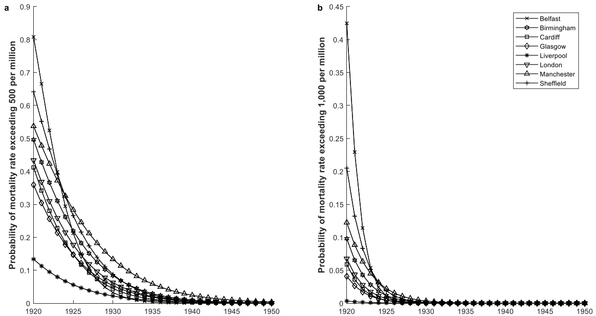
Figure B-6: Outbreak risk following the 1918-19 pandemic (One-parameter Weibull model). Outbreak probabilities computed from models fitted to each city assuming a sequence of one-parameter Weibull distributions.
