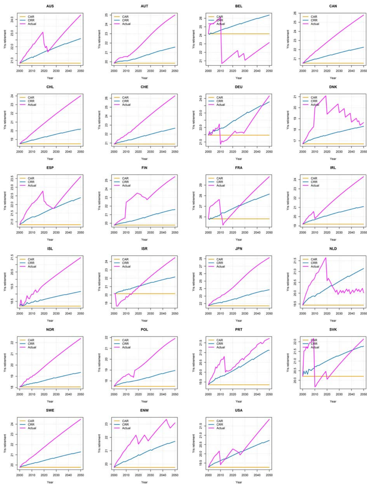
Figure 3: Forecasts of the expected years in retirement dictated by actual, CAR and CRR retirement policies
