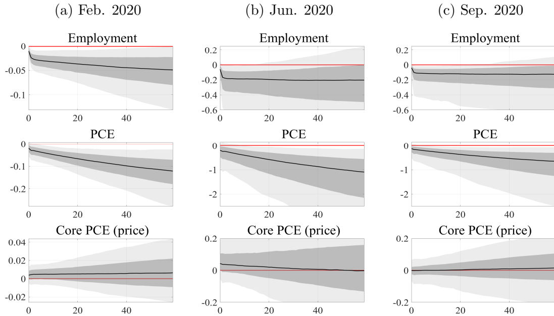
Figure 7: Median, 68 and 95 percent confidence bands of responses to unanticipated increase in the rate of unemployment from the VAR-SVt. All variables are in \text{logs} \times 100 .
