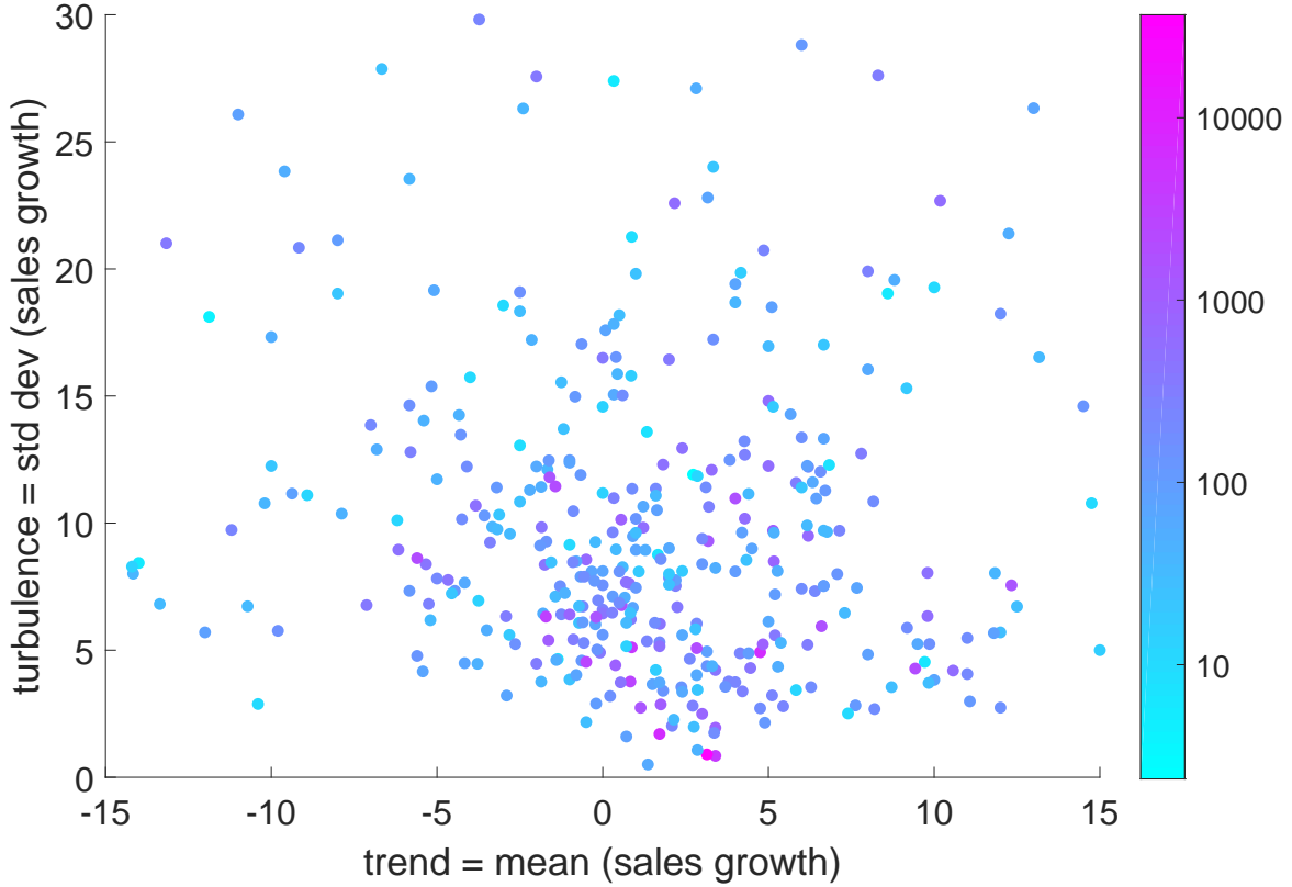
Figure 4: Scatter plot of trend and turbulence with firm size
