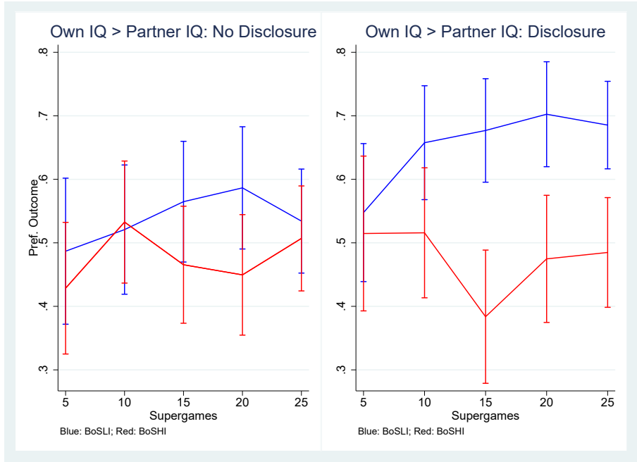
Figure 6: Battle of Sexes: Coordination on Preferred Outcome by Disclosure, Rel. Intelligence, and Game Version. The bands represent the 95% confidence intervals.
