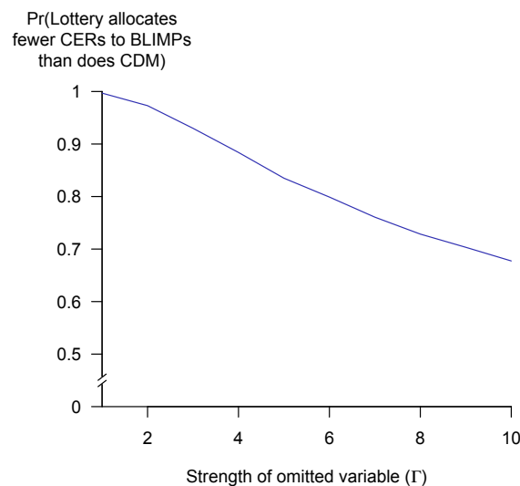
Figure 10: Sensitivity to generic omitted variable
