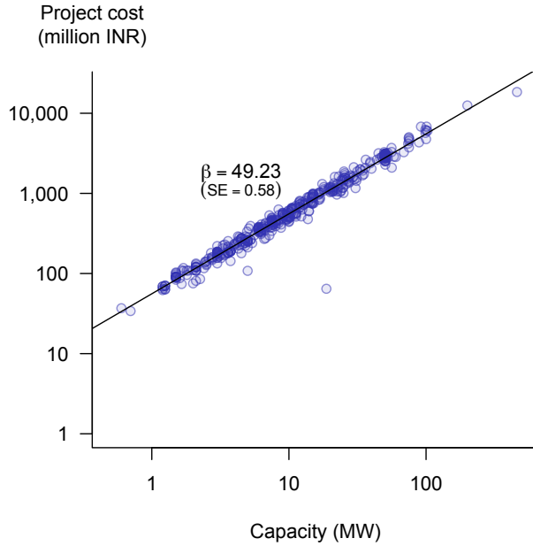
Figure 2: Capacity and project costs. Source: Bloomberg New Energy Finance
