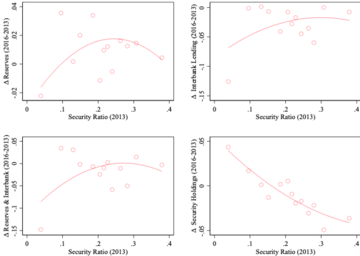
Figure 7: \Delta Bank Variables against Security Ratio
