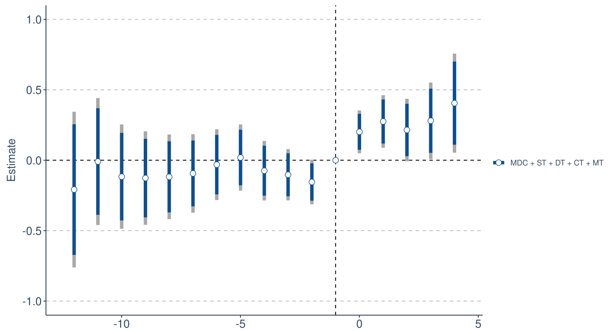
Figure 4: Event Study
