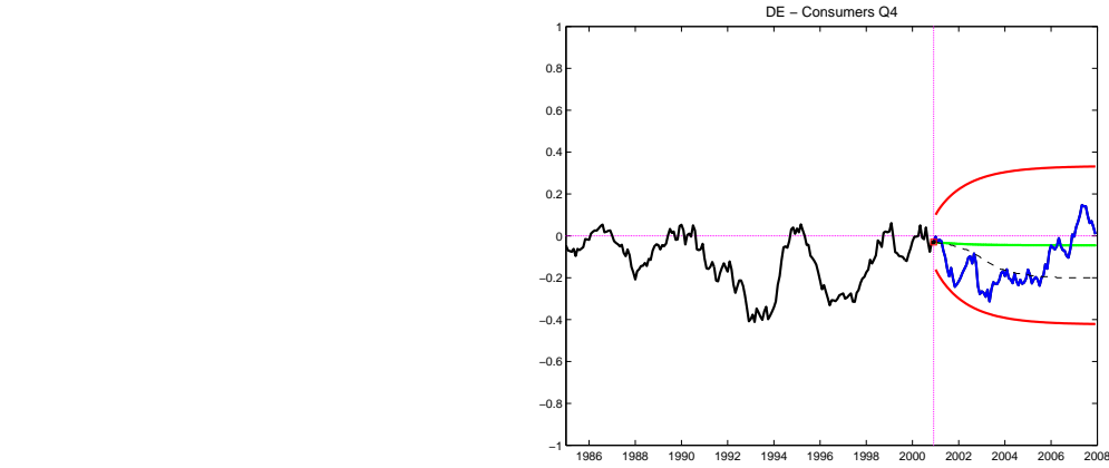
Figure 5: The evolution of the moments of the predictive density conditional on the last in-sample observation, x_0 = -0.03 , see Table 3, Consumers. The parameters are the simple averages of the two models, M1 and M2: v = .5475 , \alpha_0 = -0.0006 , \alpha_1 = 1.0109 , N = 1000 . The red bands represent the two standard deviation bounds. The green line is the (conditional) mean process. The dashed black line denotes the evolution of the global maximum.
