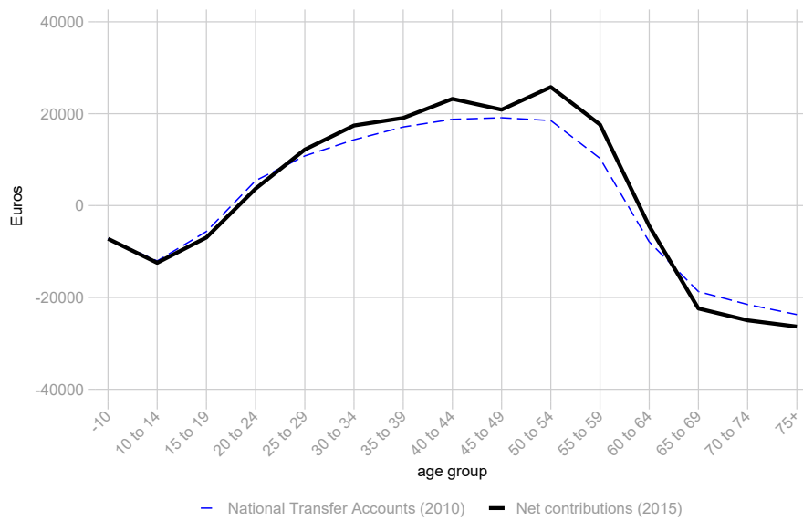
Figure 10: Validation, males
