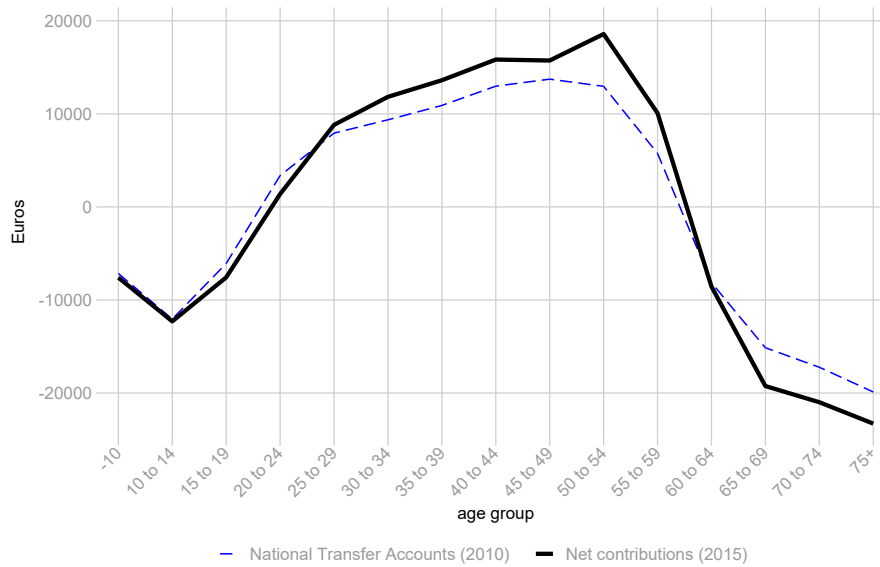
Figure 8: Validation
