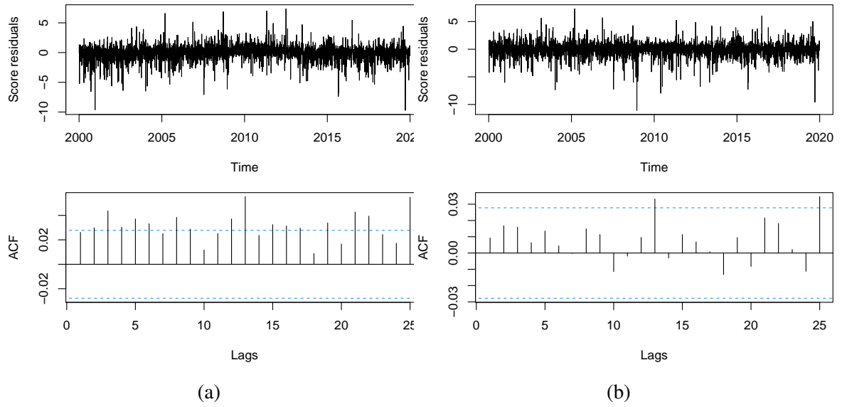
Figure 4: Panel (a) displays the conditional score residuals of the dynamic copula model of order (0,0) and their standardized empirical autocorrelation function with 95%-level confidence intervals. Panel (b) displays the conditional score residuals of the dynamic copula model of order (1,1) and their standardized empirical autocorrelation function with 95%-level confidence intervals.
