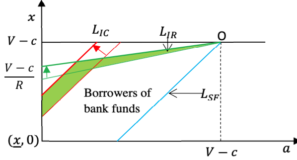
Figure 2: The effects of Simple Policy : compared to Figure 1, with R reduced due to bank funding supply enlarged, line L_{IR} rotates clockwise around point O and line L_{IC} moves northwestward. Hence, the green area marks the SMEs the policy saves.
