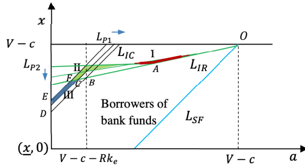
Figure D: A marginal decrease in y at y = R - 1 .
