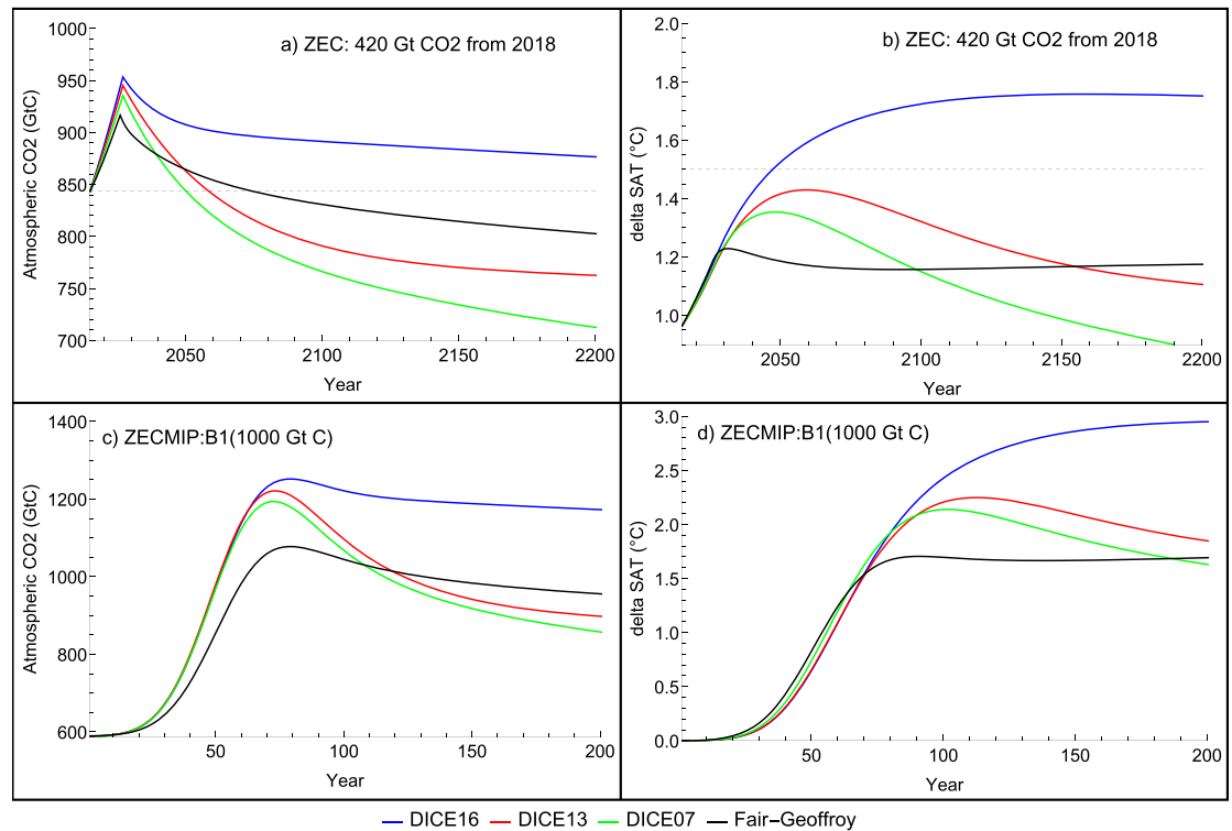
Figure 1. Zero emission commitments for different versions of DICE in comparison to FaIR-Geoffroy. The upper panel shows atmospheric carbon (a) and SAT increase (b) for cessation of emissions in 2026 after cumulative emissions of 420 Gt CO 2 since 2018 have been reached. The lower panel shows the corresponding information for a bell-shaped emission path with cumulative emissions of 1000 Gt C, starting at preindustrial conditions (ZECMIP:B1). Both panels show the CO 2 -only responses, forcing of other non-CO 2 -gases is not included.
