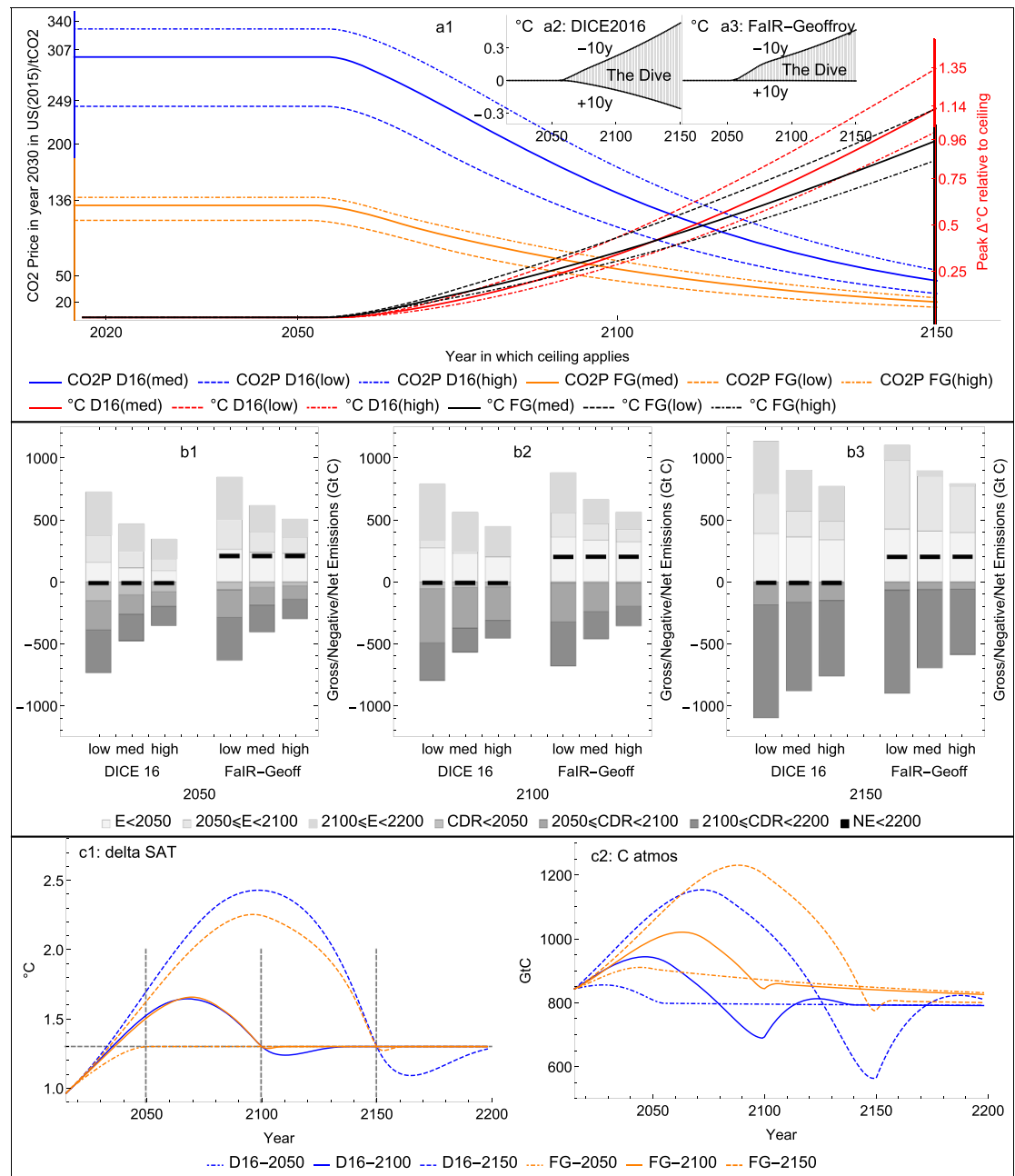
Figure 2. Implications of optimal overshoot climate policies. The upper panel shows the CO 2 -price in the year 2030 and how much temperature increases above the temperature ceiling, both in dependence of the compliance date (a1); (a2) and (a3) show the 'Dive', i.e. the temperature difference to ceiling 10 years before and 10 years after the ceiling has become binding, again in dependence of compliance date, here for the low CDR cost scenario. The middle panel shows the distribution of gross emissions, CDR, and net emissions for three selected compliance dates, 2050 (b1), 2100 (b2), and 2150 (b3). The lower panel shows the profile of SAT temperature and atmospheric CO 2 for a ceiling of 1.3 °C with compliance in 2050, 2100, and 2150 for medium CDR costs. All information are provided for both specifications for the carbon cycle and climate dynamics, DICE2016 (D16) and FaIR-Geoffroy (FG).
