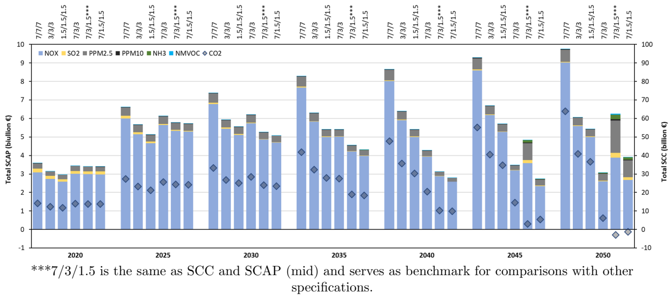
Figure 4: Total SCAP and SCC for different discount and interest rates
