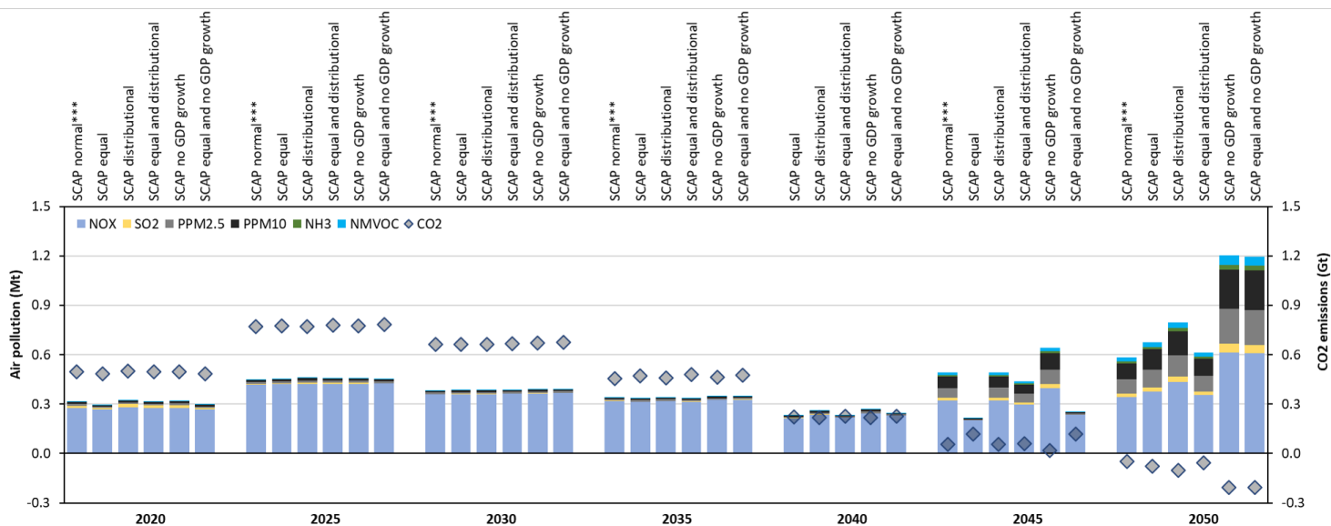
Figure C.20: Air pollutant and carbon emissions for different SCAP specifications
