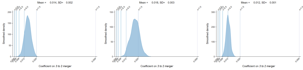
(a) Uniform(1.0, 3.5) (b) Beta(0.5, 0.5)*2.5+1 (c) Beta(2, 2)*2.5+1
