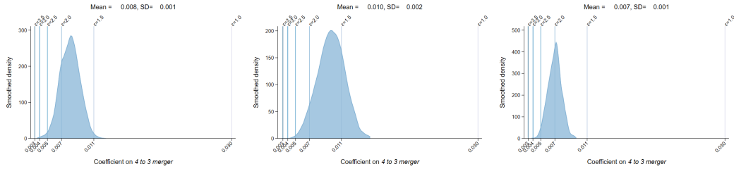
(a) Uniform(1.0, 3.5) (b) Beta(0.5, 0.5)*2.5+1 (c) Beta(2, 2)*2.5+1
