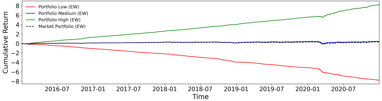
Figure 9: Portfolios Cumulative Returns of Sorting Lead Return \mathcal{LR}(\omega_{ij,t-365:t}) S&P500 constituents are sorted into quintile equal-weighted portfolios. The three solid lines in red, blue, green refer to cumulative returns of portfolios with lowest, medium, and highest lead return value. The black dash line is the benchmark cumulative return of an equal-weighted S&P500 market portfolio.
