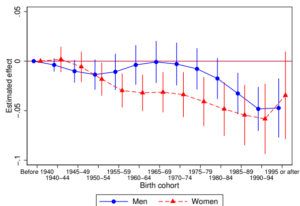
Figure 7: Estimated birth-cohort effects by gender
