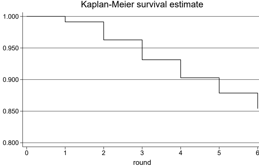
Figure 1: Non-parametric survival
