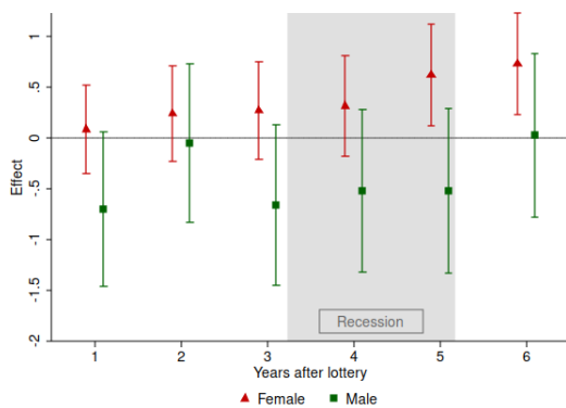
(c) Cohort 1: female vs male applicants
