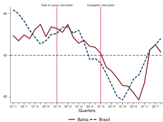
(b) Cohort 2: Start in Mar-2013 and completion in Dec-2014
