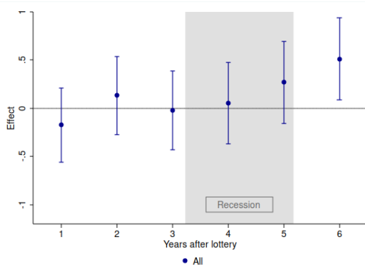
(a) Cohort 1: all applicants
