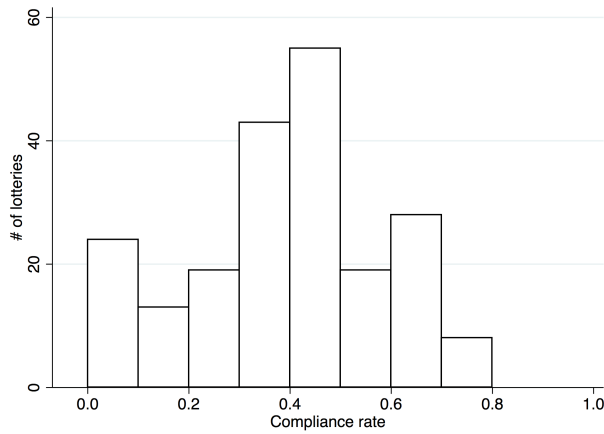
(a) Cohort 1: 190 wait lists
