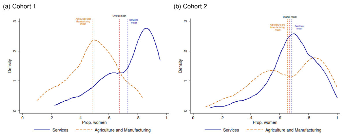
Figure 6: Distribution of the proportion of female applicants by the type of course
