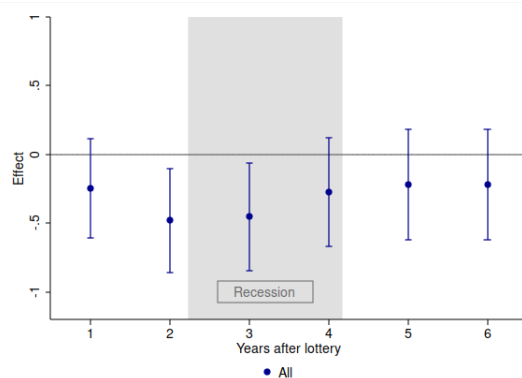
(b) Cohort 2: all applicants
