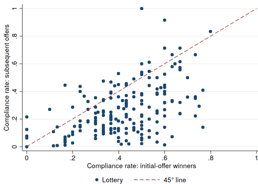
Figure A2: Take-up rate among lottery winners and wait list
