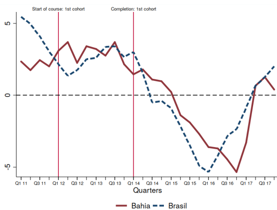
(a) Cohort 1: Start in Mar-2012 and completion in Dec-2013
