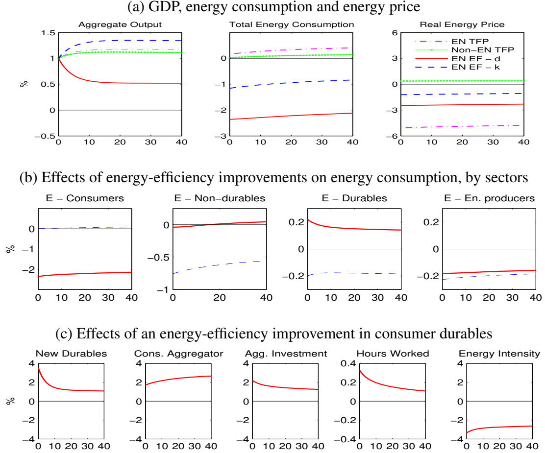
Figure 7: Impulse responses from the E-DSGE model
