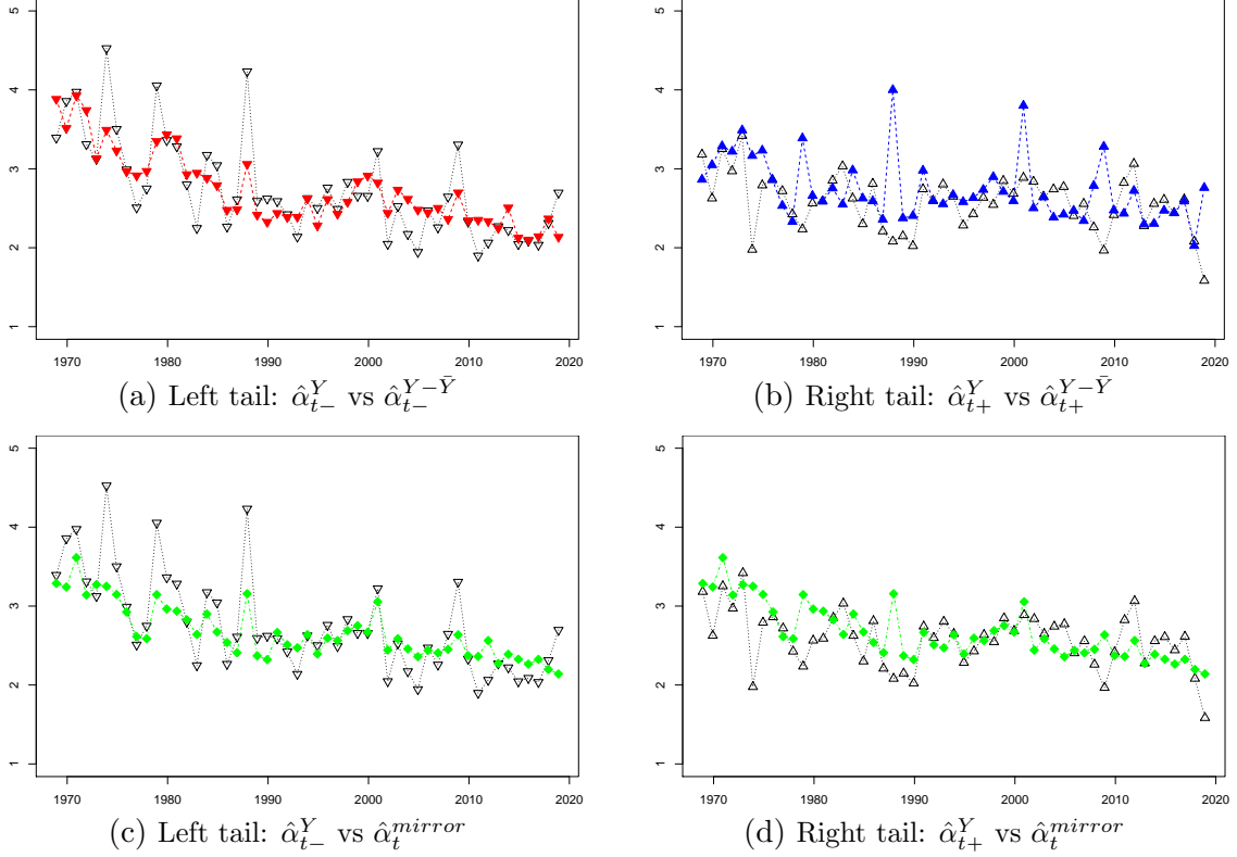
Figure 5: Bias-corrected \hat{\alpha}
