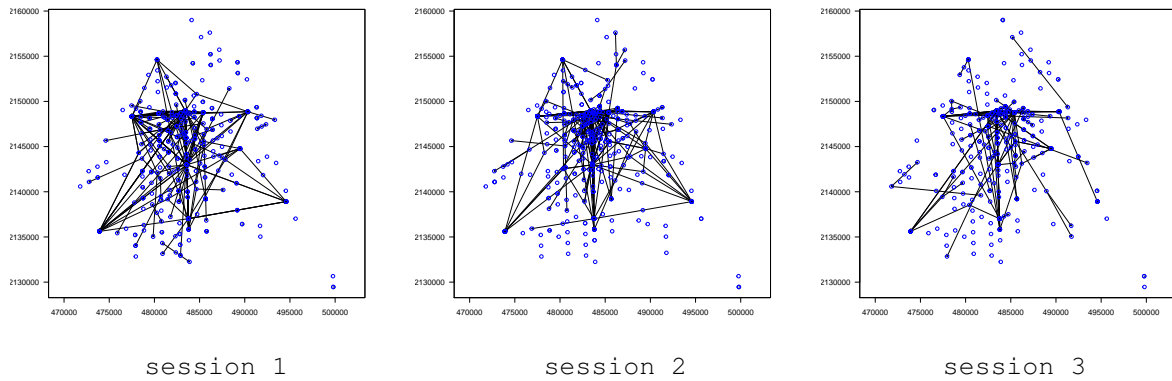
Figure 3: The capture history was constructed from the data collected on social media in Mexico City. Each blue circle represents the cell/trap centroid, and the directed arrows connect pairs of traps where SMUs were captured and recaptured on the indicated observation day, where session 1 corresponds to June 22, session 2 corresponds to June 23, and session 3 corresponds to June 24. The circles with a dot at the centre indicate that the user was captured only by that trap while those without a dot indicate that no user was captured on that day.
