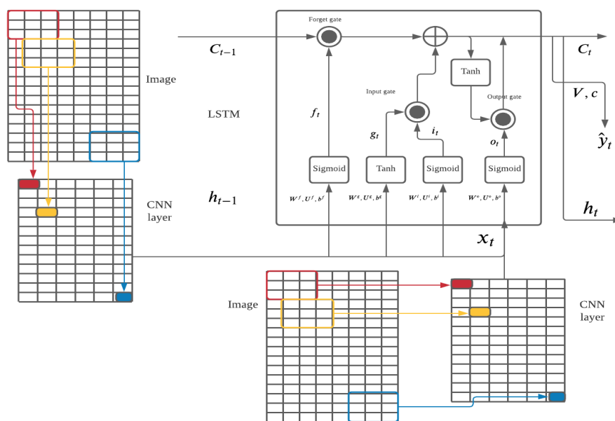
Figure 2. Architecture of ConvLSTM2D in one layer.
