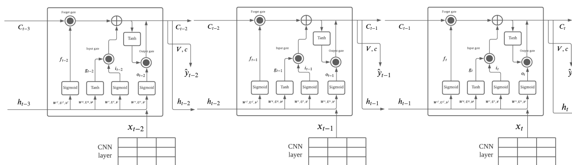
Figure 3. Entire architecture of ConvLSTM2D.
