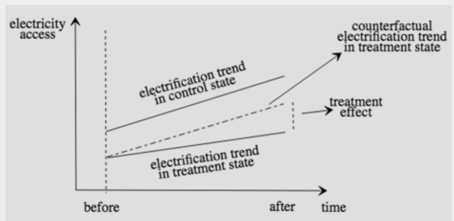
Figure 2: Selection Bias
