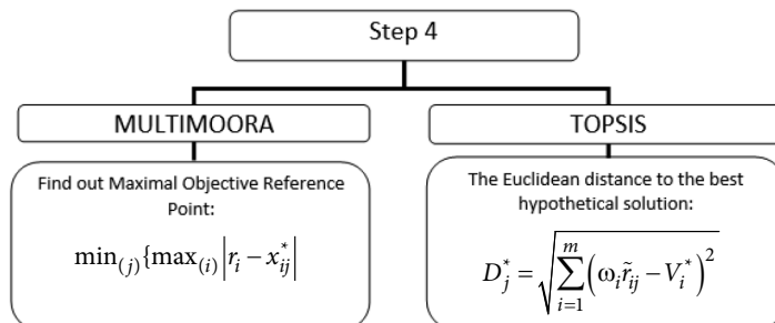
Figure 6. The reference point for each criterion using MULTIMOORA and TOPSIS methods (source: developed by authors based on Brauers & Zavadskas (2012))
