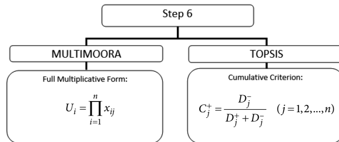
Figure 8. Full-multiplicative form for MULTIMOORA method and relative closeness coefficient for TOPSIS method (source: developed by authors based on Brauers and Zavadskas (2012))
