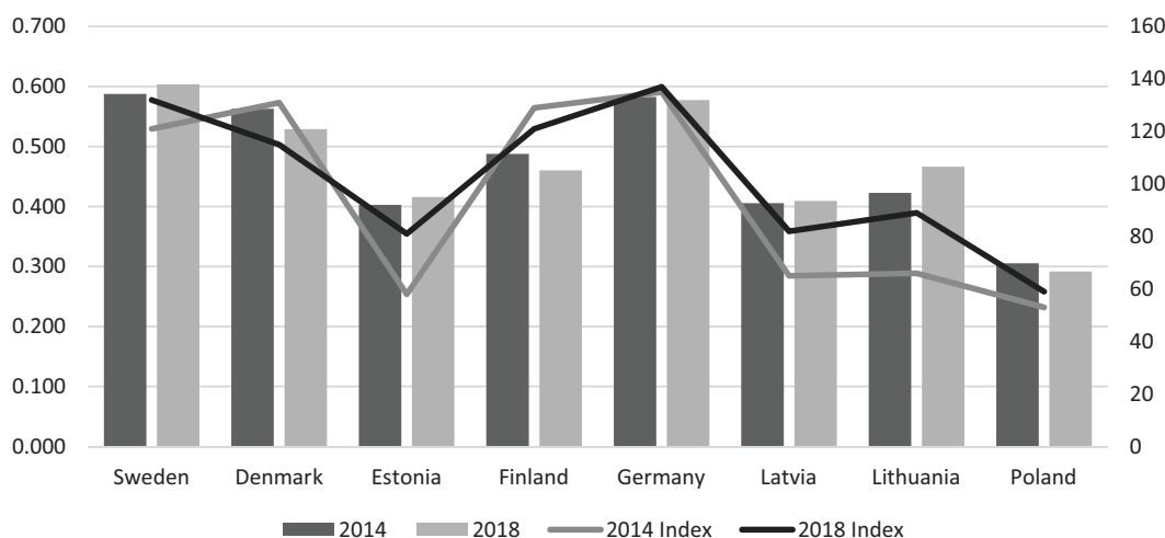
Figure 15. Development of eco-innovation in Baltic Sea Region in the period of 2014–2018 represented by TOPSIS and eco-innovation index (source: developed by authors)
