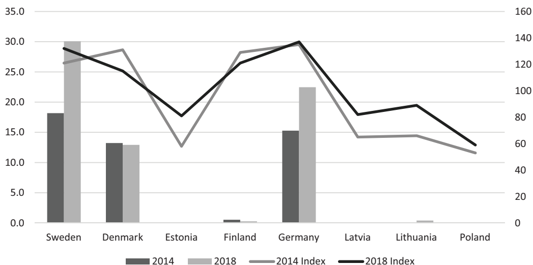
Figure 14. Development of eco-innovation in Baltic Sea Region in the period of 2014–2018 represented by MULTIMOORA and eco-innovation index (source: developed by authors)
