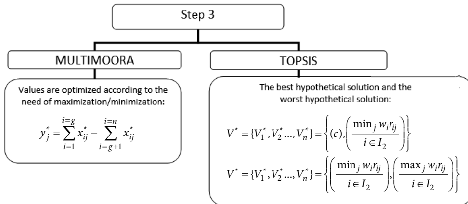
Figure 5. Maximization and minimization of criteria using TOPSIS and MULTIMOORA methods (source: developed by authors based on Brauers & Zavadskas (2010))
