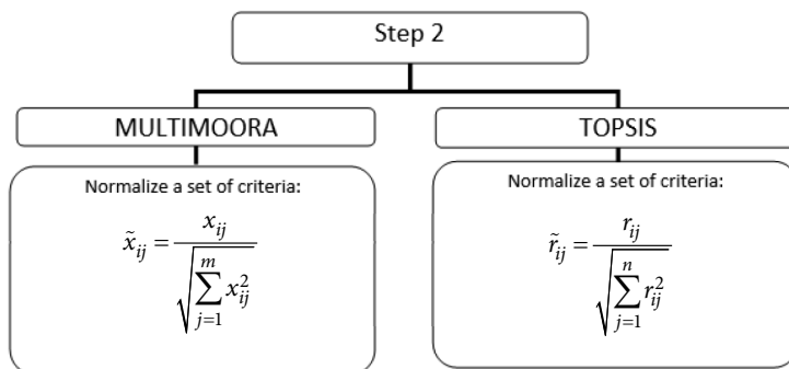
Figure 4. Normalization of the criteria by TOPSIS and MULTIMOORA methods (source: developed by authors based on Byun & Lee (2005))
