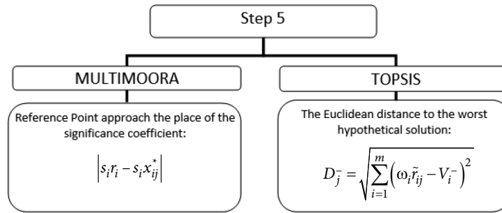
Figure 7. Deviation of normalized values using MULTIMOORA and TOPSIS methods (source: developed by authors based on Brauers & Zavadskas (2012))
