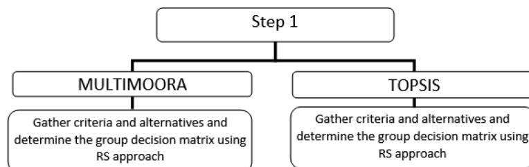
Figure 3. Decision matrix creation for TOPSIS and MULTIMOORA methods (source: developed by authors based on Brauers & Zavadskas (2010))
