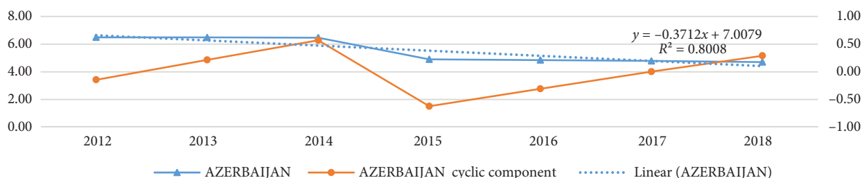
Figure 2. Visualization of the input time series of the BASEL AML INDEX, trend and cyclic components in the context of Azerbaijan for the period from 2012 to 2018 (source: authors' calculation)
