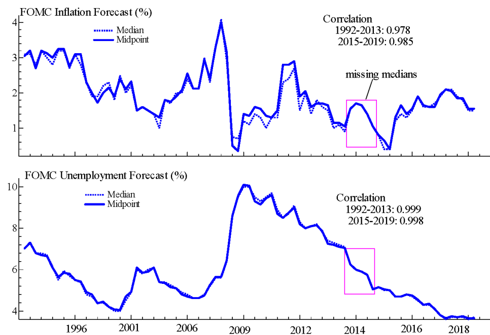
Figure 2. Median and midpoint of FOMC forecast distributions.
