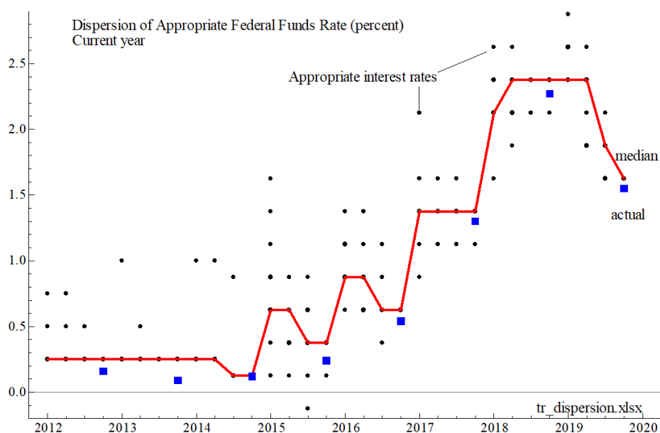
Figure 1. Appropriate federal funds rates for the end of the current year. Participants' forecasts are shown as black circles; the median of the forecast distributions are shown in red; the actual values of the federal funds rate in Q4 of each year are shown as blue squares.
