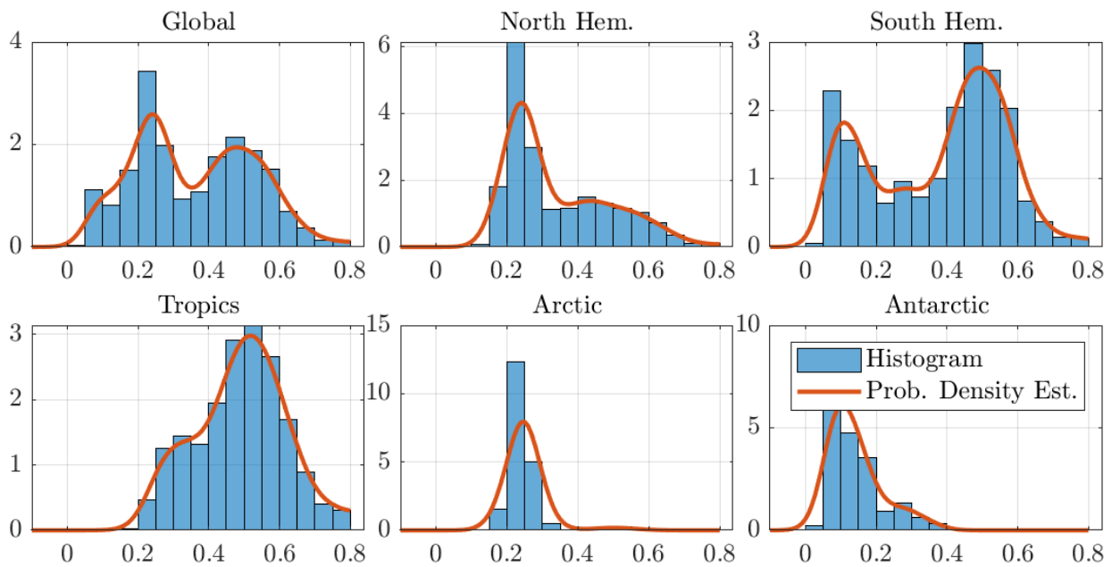
Figure A7. Histograms and probability density estimates of long memory estimates for monthly individual grid observations of temperature anomalies. We use the optimal bandwidth, the 1200 km smoothing radius dataset, and the FELW estimator.
