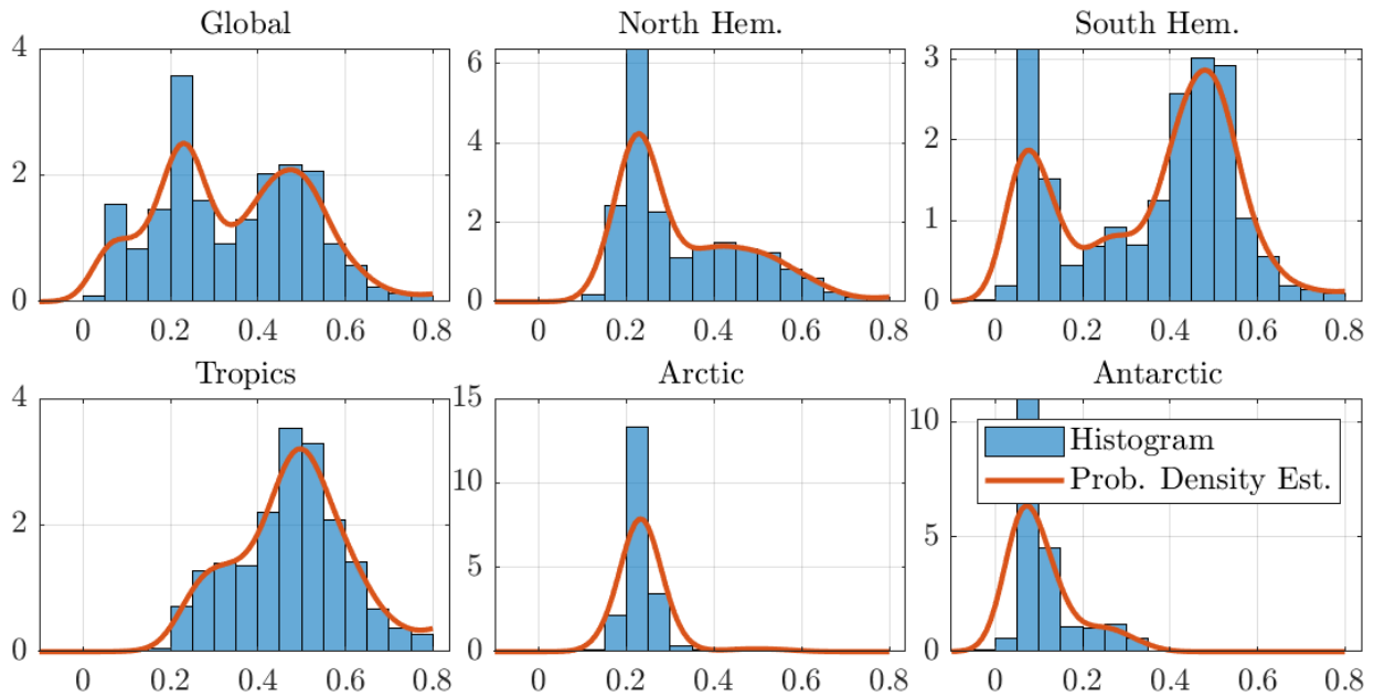
Figure A6. Histograms and probability density estimates of long memory estimates for monthly individual grid observations of temperature anomalies. We use the optimal bandwidth, the 1200 km smoothing radius dataset, and the LW estimator.
