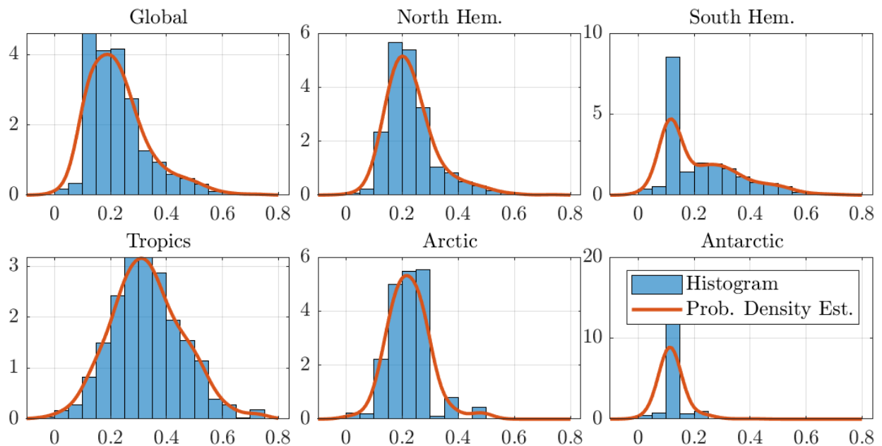
Figure A9. Histograms and probability density estimates of long memory estimates for monthly individual grid observations of temperature anomalies. We use the optimal bandwidth, the 250 km smoothing radius dataset, and the LW estimator.
