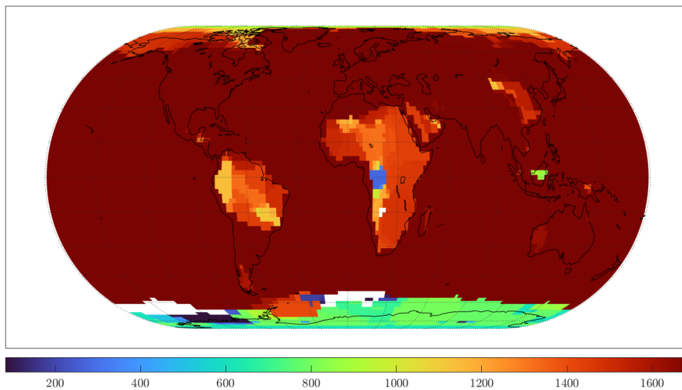
Figure A2. Author’s own plot with data from GISTEMP. Smoothing radius of 1200 km.
