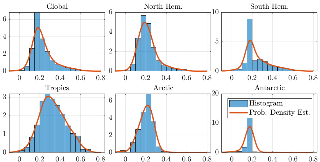
Figure 8. Histograms and probability density estimates of long memory estimates for monthly individual grid observations of temperature anomalies. We use the optimal bandwidth, the 250 km smoothing radius dataset, and the log-periodogram regression (GPH) estimator.
