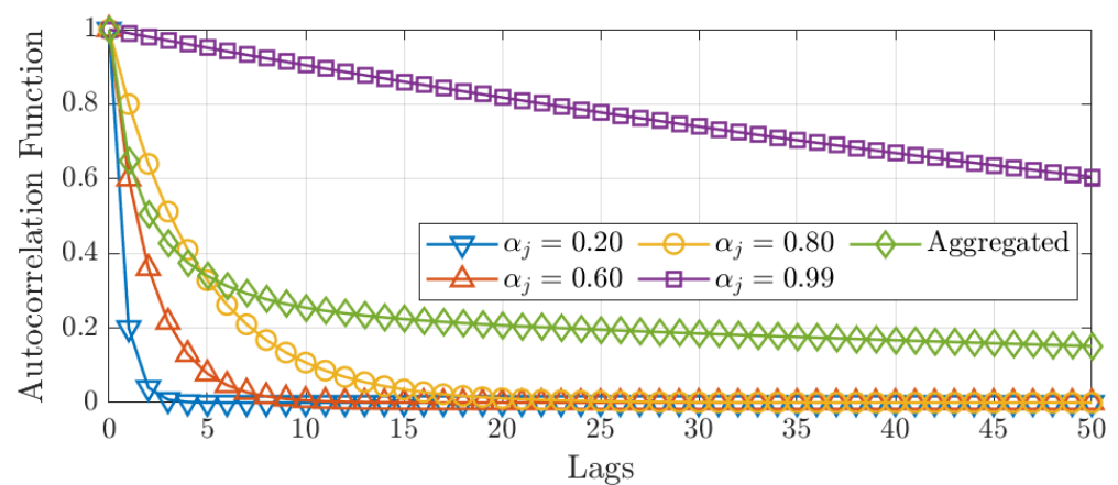
Figure 4. Autocorrelation functions for individual AR(1) processes with different autoregressive coefficient. Also shown, the autocorrelation function of the aggregated process.
