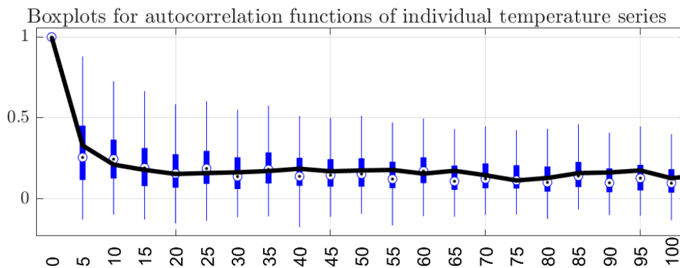
Figure A1. Boxplots for autocorrelation functions of individual temperature series. On each box, the central mark indicates the median, and the bottom and top edges of the box indicate the 1st and 3rd quartiles, respectively. The whiskers extend to approximately 99.3% coverage if the data are normally distributed. Also shown in a black line, the autocorrelation function for the temperature at the grid near London ( 51^{\circ}, -1^{\circ} ).
