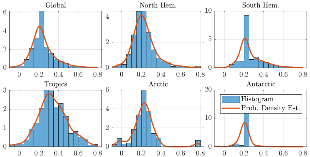
Figure A8. Histograms and probability density estimates of long memory estimates for monthly individual grid observations of temperature anomalies. We use the optimal bandwidth, the 250 km smoothing radius dataset, and the AG estimator.
