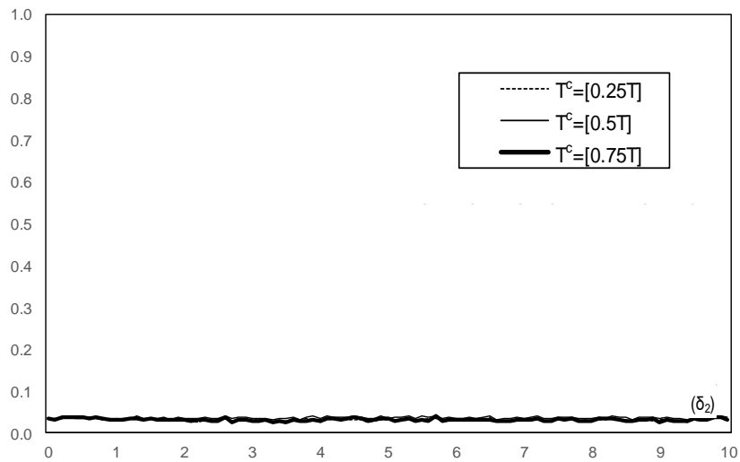
Figure 9. Size of the sup-LR 2,T test for a variance change accounting for a coefficient change.
