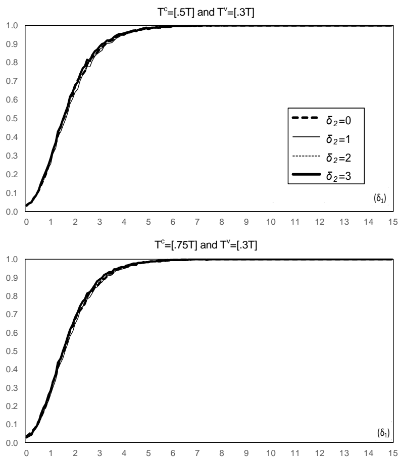
Figure 10. Power of the sup-LR 2,T test for a variance change accounting for a coefficient change.
