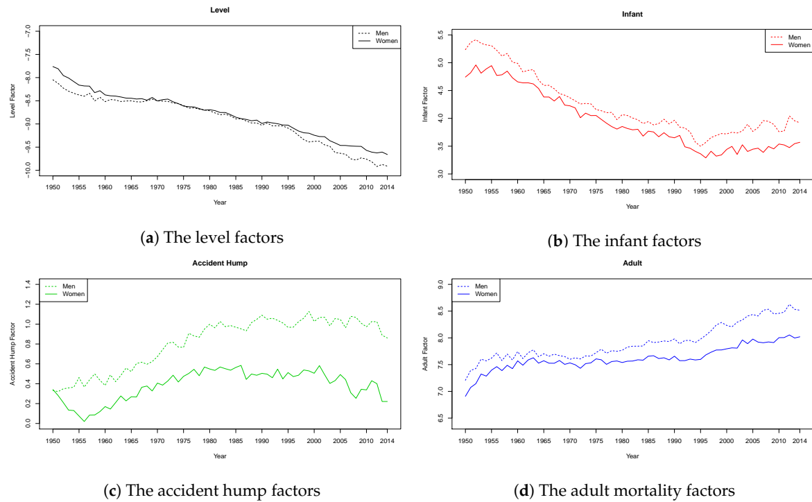
Figure 5. The factors \kappa_{i,t} , i = 0, 1, 2, 3 estimated by the two-step procedure for France using data from 1950–2014. The plots are showing the level factor, infant factor, accident hump factor, and adult factor for both genders, respectively.
