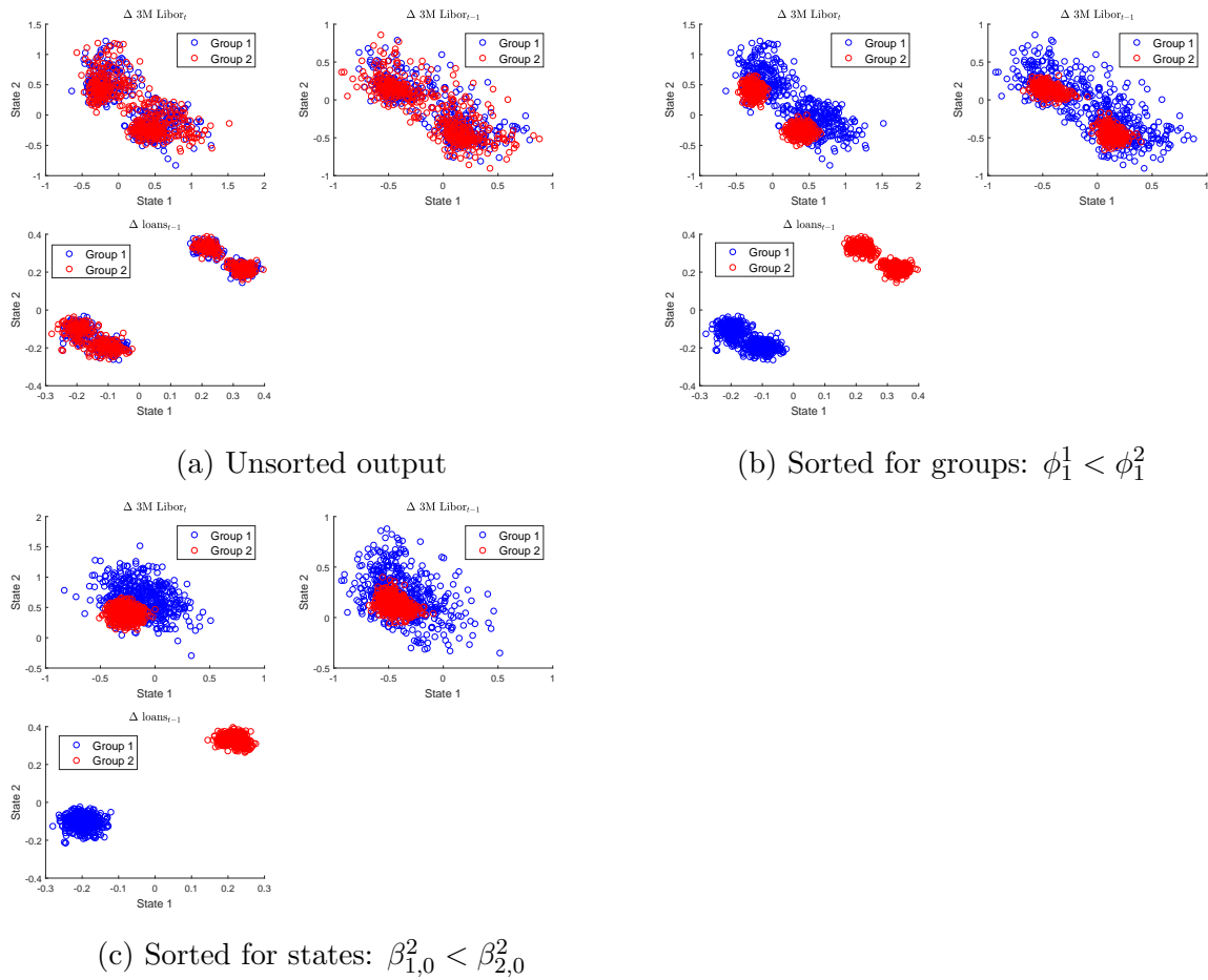
Figure 8 – Posterior processing. Scatter plots of group-specific parameters for State 1 against those for State 2.
