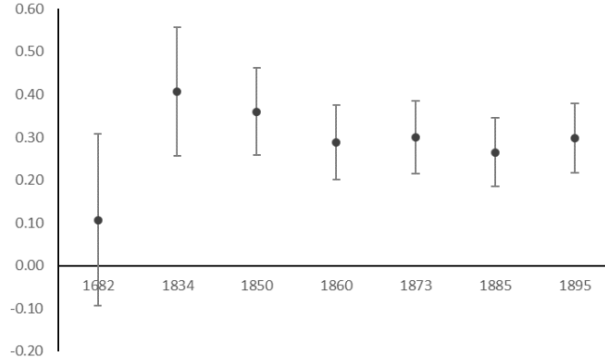
Figure 4: Coefficients from second stage estimations, 1682 to 1895. Dependent variable: \ln(\textit{Theil}) , instrument: share of boulder clay , controls included.
