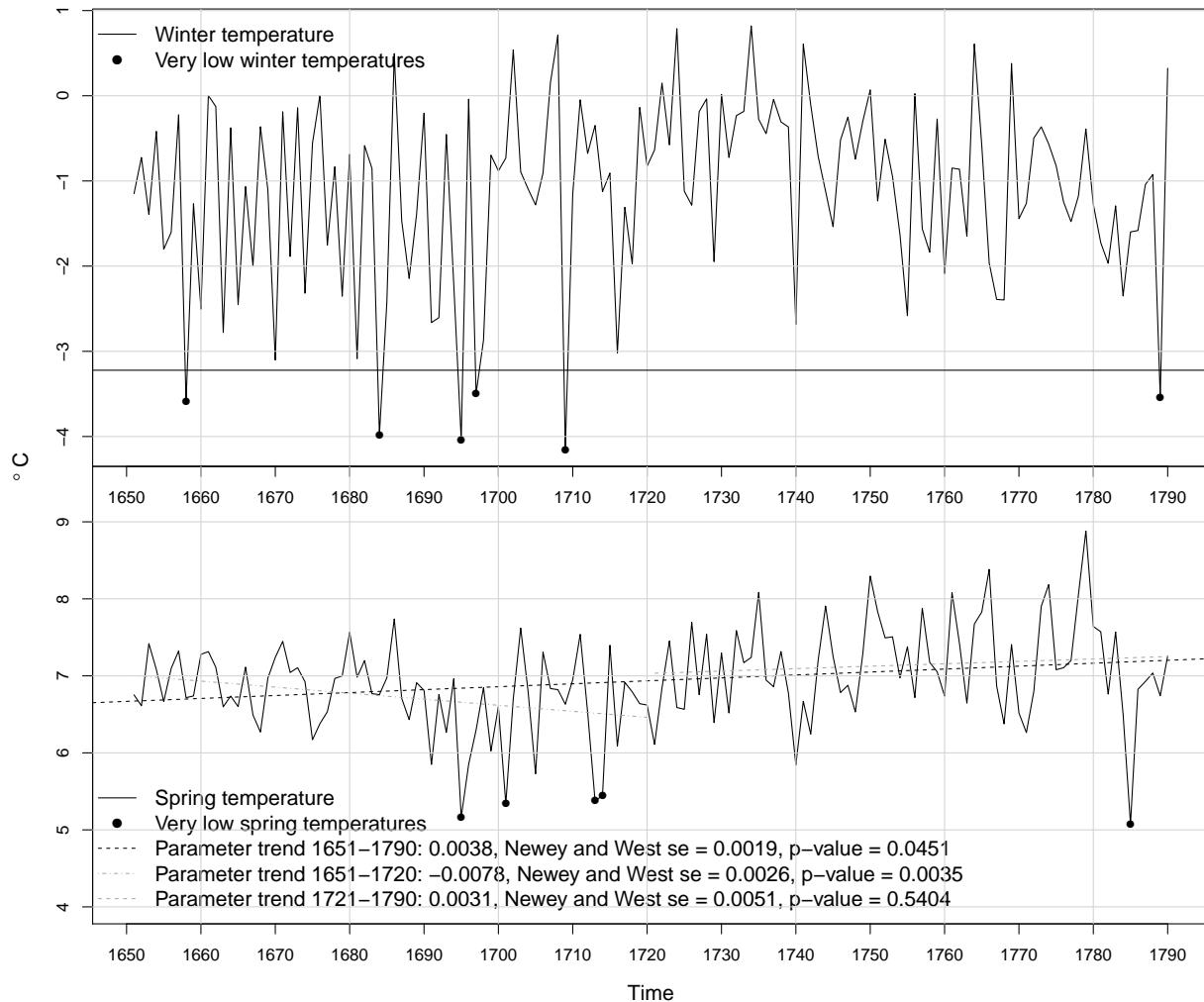
Figure S7: Temperature reconstructions for Europe 1651–1790. Very low: < mean minus two times the standard deviation. Own representation. Horizontal line in upper panel is drawn at the average winter temperature of 1963 ( -3.22^{\circ}\text{C} ), when major rivers (Elbe, Rhine, Main) were frozen. Data sources: Luterbacher et al. (2004); Xoplaki et al. (2005); data retrieved from NOAA (2017).
