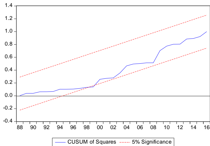
Figure 2. Plot of CUSUMQ test for equation (3)
