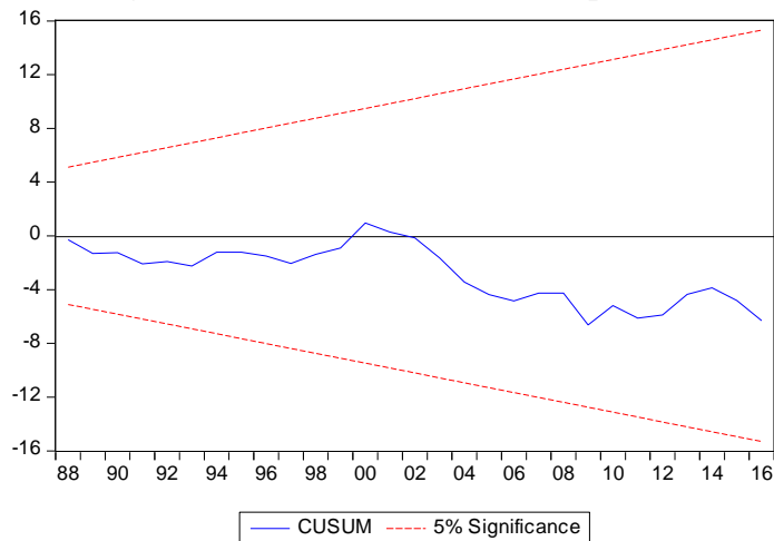
Figure 1. Plot of CUSUM test for equation (3)
