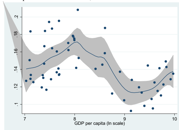
Figure A.2. Semiparametric estimates, alternative measures of inequality: Gini
