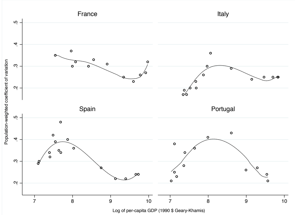
Fig. 4. Regional income dispersion (WCV) and per-capita GDP (All sample, 1860-2010)
