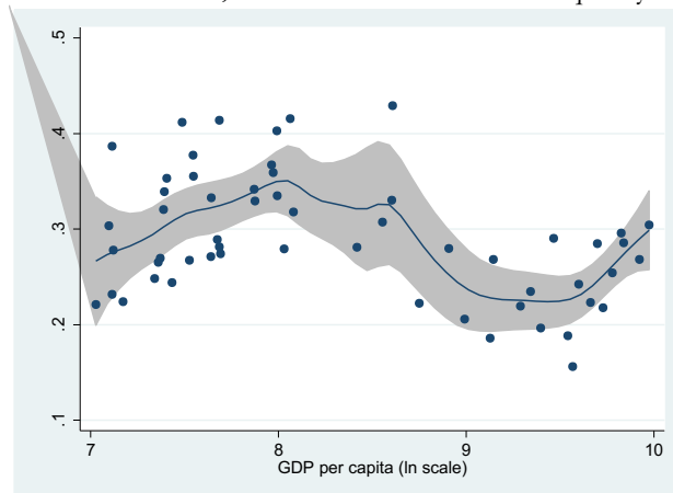
Figure A.1. Semiparametric estimates, alternative measures of inequality: coefficient of variation
