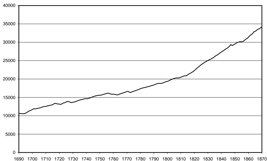
Figure 4: The trajectory of ln real wage (vertical axis) and ln population size (horizontal axis).
