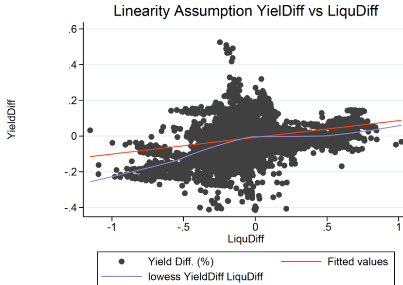
Figure 6. Linearity in parameters
