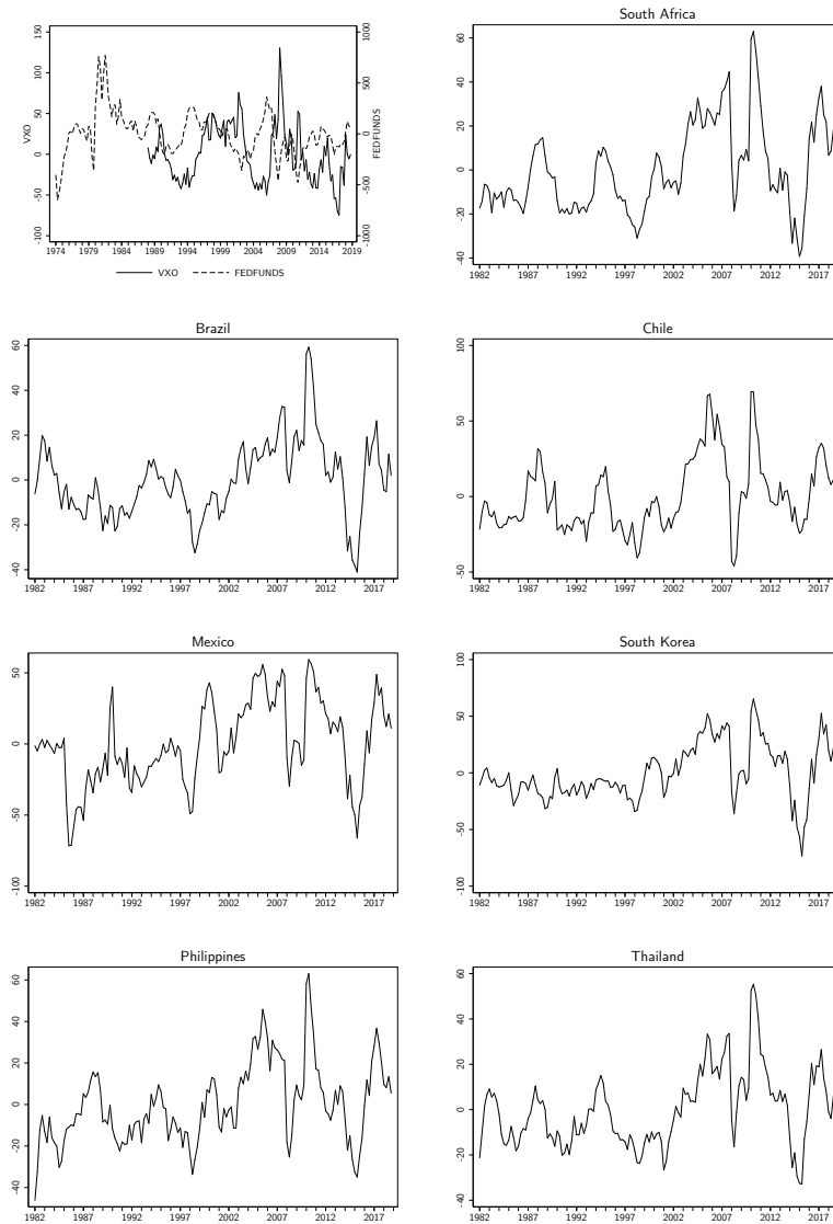
Figure 3: Real federal funds rate and VIXO (upper left panel) and country-specific commodity terms of trade (remaining panels), cyclical components
