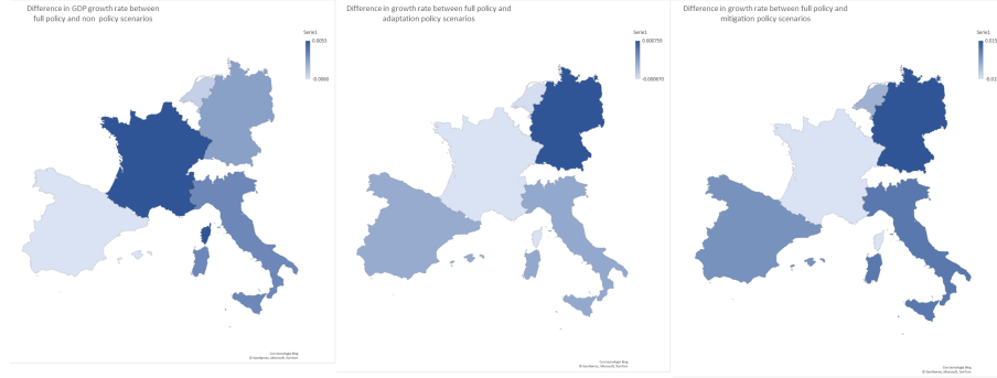
Figure 4: Difference in optimal GDP growth rate with full environmental policy and: (i) no policy (left panel), (ii) only adaptation policy (central panel), and (iii) only mitigation policy (right panel).
