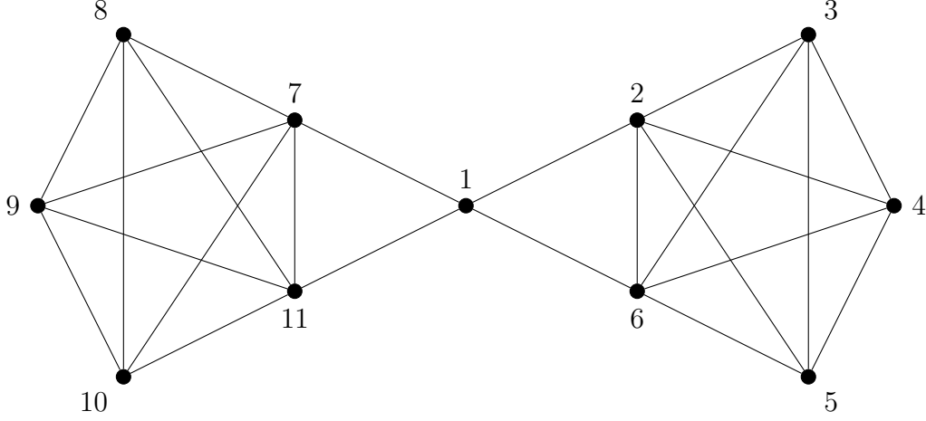
Figure 1. 11-players network
