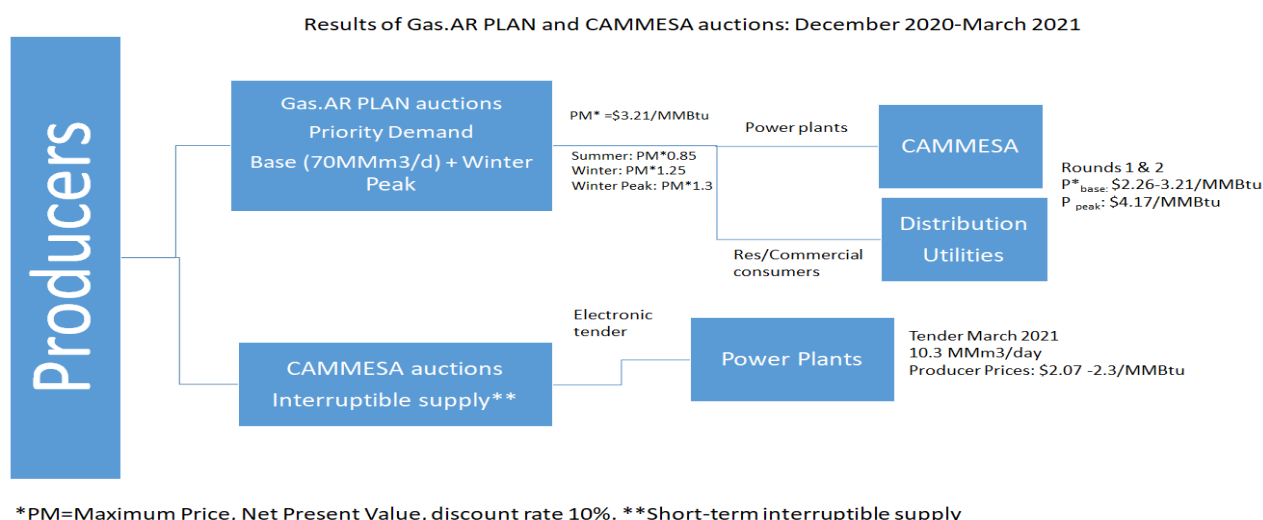
Figure 7: Argentine Producers Prices Gas.AR PLAN and short- term supplies 19
