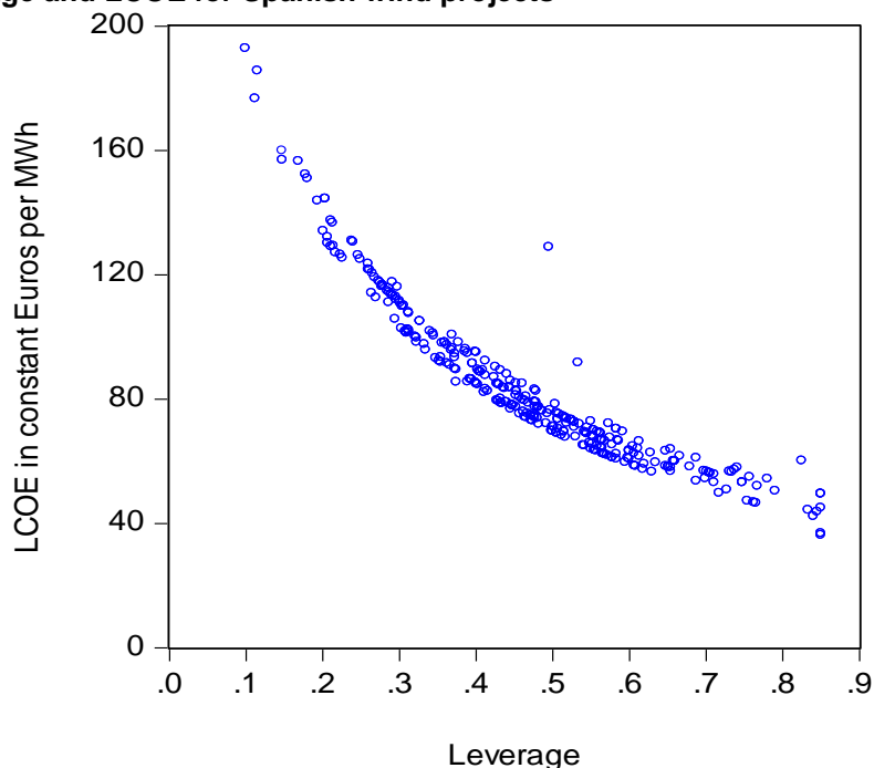
Figure 2: Leverage and LCOE for Spanish wind projects
