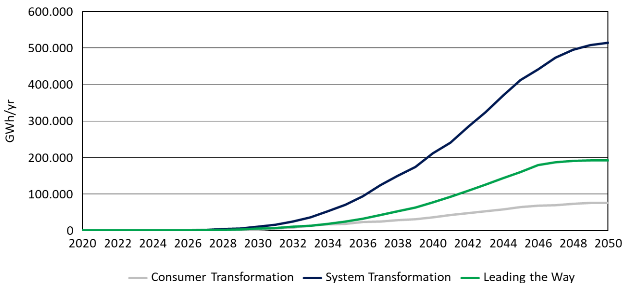
Figure 15: UK total hydrogen demand by scenario
