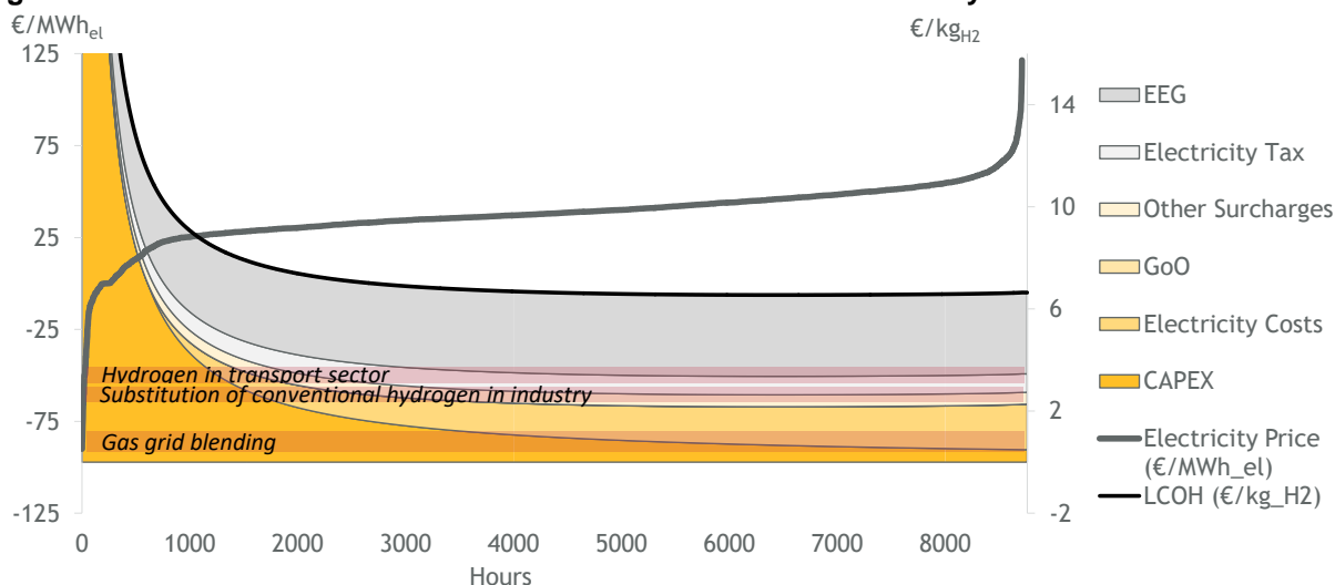
Figure 10: LCOH and cost benchmarks on the demand side in Germany in 2019
