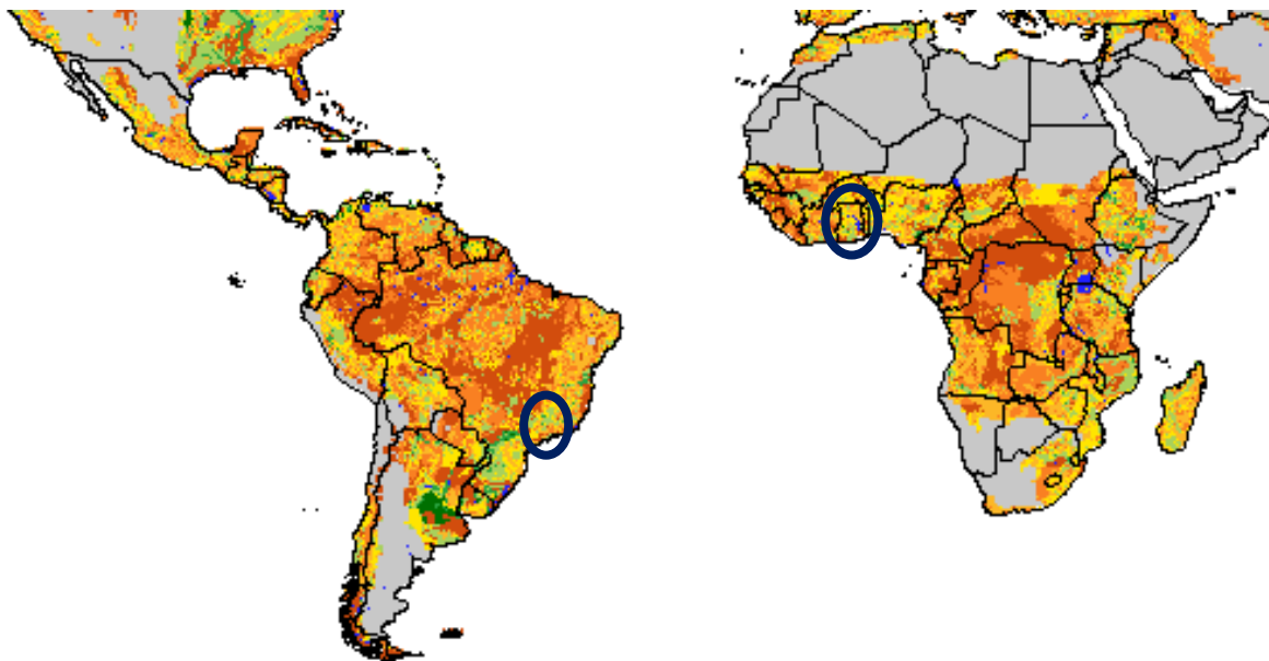
Figure 1: Global net primary productivity Source: http://www.usf.Uni-Osnabrueck.DE/~hlieth
