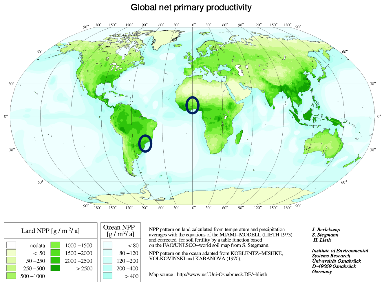
Figure 1: Global net primary productivity Source: http://www.usf.Uni-Osnabrueck.DE/~hlieth
